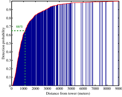
Figure 6: Cumulative distribution of phone-tower distances based on the reports.
