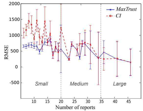
Figure 9: Error of CI and MaxTrust according to the number of reports for different cell towers.
