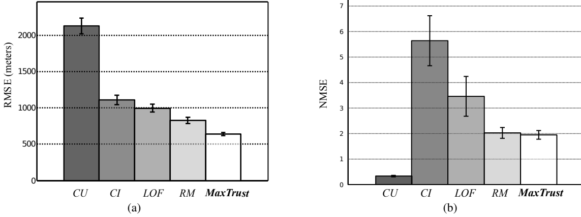
Figure 7: Bar plots of the RMSE (a) and NMSE (b) scoring the predictions of cell tower locations for the five algorithms.
