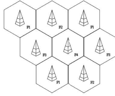
Figure 5: Topology of a cellular network for omni-directional masts.
