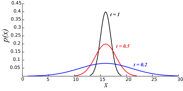
Figure 2: Scaling effect of the trustworthiness parameter on a Gaussian estimate.
