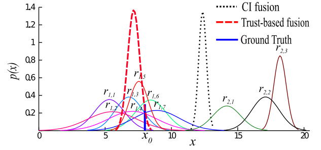
Figure 3: Example of a set of 10 reports of two users (user 1 and 2) fused through the CI fusion and the trust-based fusion.
