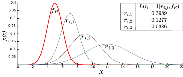
Figure 4: Likelihood values of three reports given the fused estimate f .
