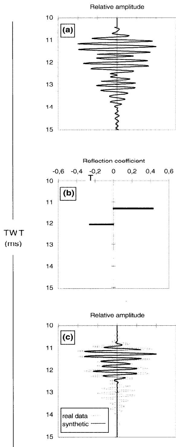
Fig. 6. (a) Single trace over the a buried portion of The Invincible . (b) Model incorporating reflection coefficients calculated for the sea bed and the wreck reflector. (c) Synthetic trace (black) produced by convolving the Klauder wavelet with the model. Note the excellent fit between the observed data (grey) and the synthetic.
