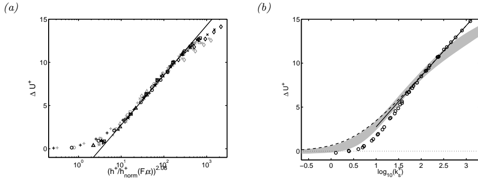
FIGURE 5. (a) Roughness function for different roughness factors and different shape functions plotted versus normalised and exponentiated roughness height parameter (symbols as in figure 3); the black line shows the fully rough asymptote. (b) Comparison of rescaled roughness data (shaded region) with Nikuradse (1950) sand grain roughness data (black circles) and the Colebrook interpolation formula (4.4) (black dashed line). The fully rough asymptote is shown by the continuous black line.
