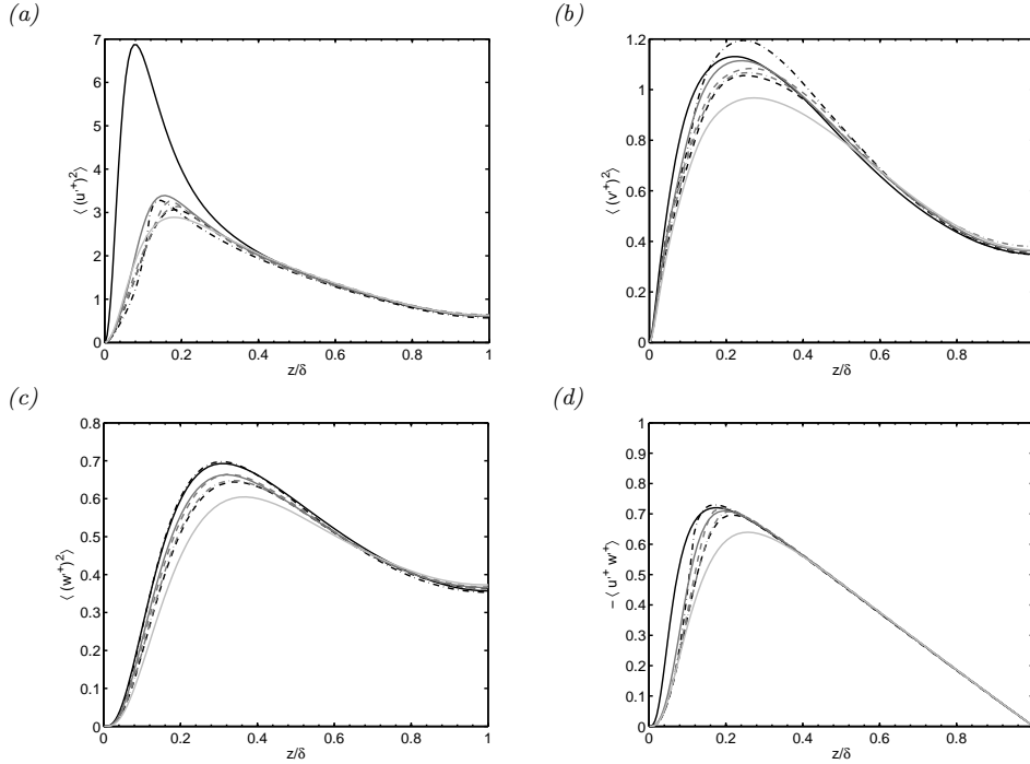
FIGURE 10. Profiles of Reynolds stresses for different shape functions using a roughness factor \alpha = 1 , and height parameter h^+ = 10 . (a): streamwise normal stress; (b): spanwise normal stress; (c): wall-normal stress; (d): shear stress. Line styles as in figure 8.
