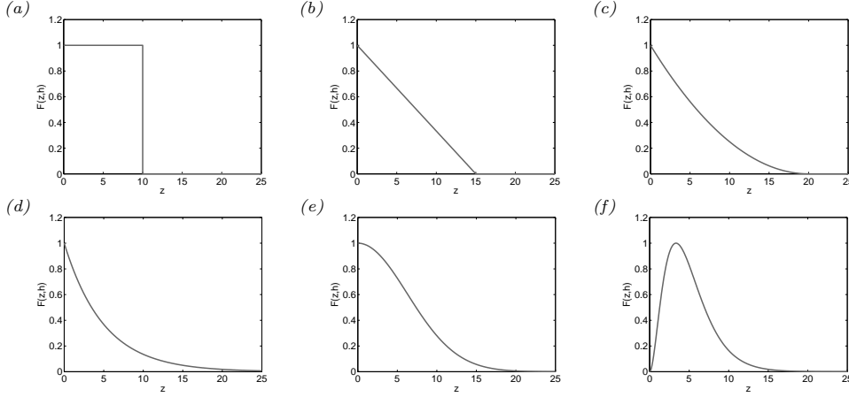
FIGURE 1. Different types of shape functions used to simulate roughnesses in this paper; (a) box, (b) triangular, (c) parabolic, (d) exponential, (e) Gaussian and (f) orbital shape function. All shape functions are based on the same roughness height parameter h = 5 .
