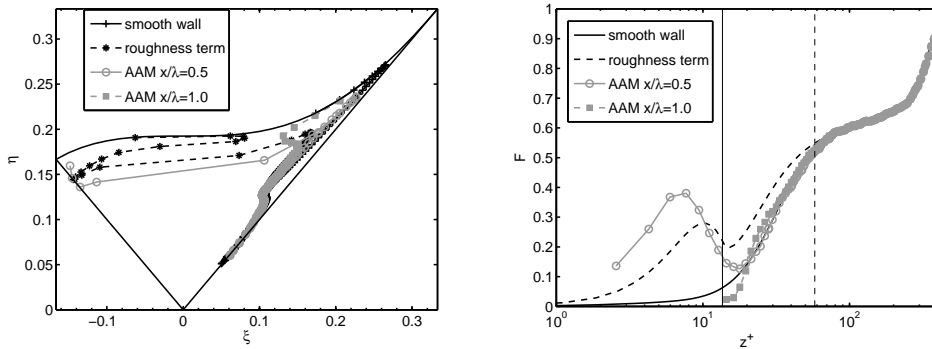
FIGURE 19. Direct comparison with AAM: Anisotropy of the Reynolds stresses. (a) anisotropy invariant map, (b) invariant F . The thin black continuous vertical line indicates the height of the roughness elements. The thin black dashed vertical line indicates the extent of the roughness sublayer as estimated by AAM.
