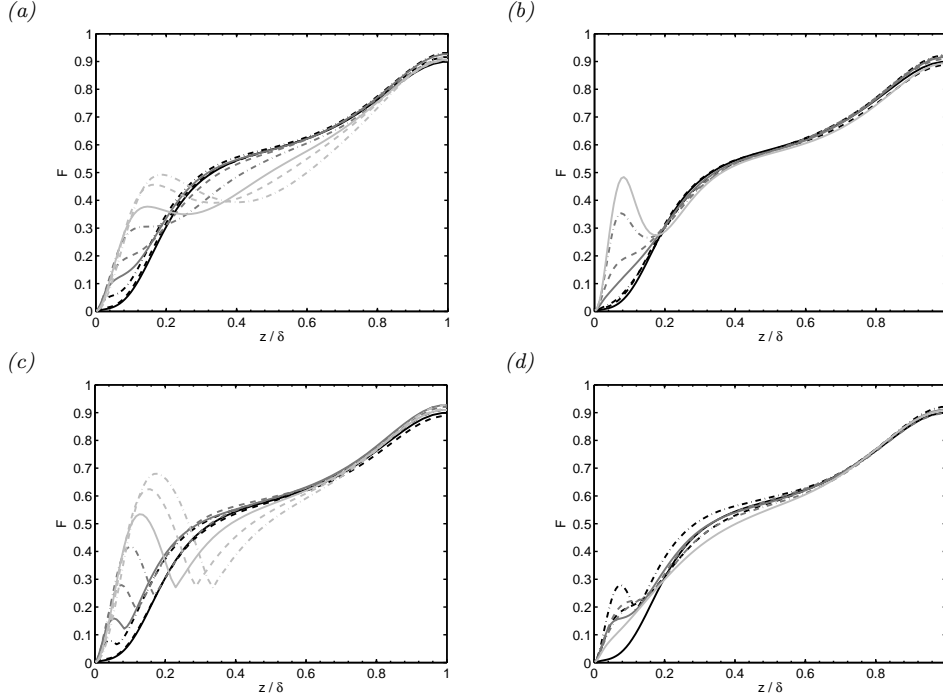
FIGURE 12. Invariant function F . (a) Gaussian shape function, \alpha = 1 , different roughness heights (line styles as in figure 6 (a)). (b) Gaussian shape function, h^+ = 10 , different roughness factors (line styles as in figure 6 (b)). (c) box shape function, \alpha = 1 , different roughness heights (line styles as in (a)). (d) various shape function using \alpha = 1 , h^+ = 10 (line styles as in figure 8).
