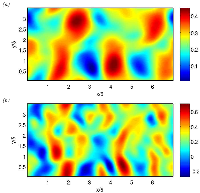
FIGURE 16. Contours of u at a distance of z^+ = 10 from the wall in two extremely rough cases ( \alpha = 10 , h^+ = 30 ). (a) Gaussian shape function, (b) box shape function.
