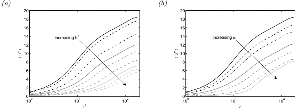
FIGURE 6. Mean streamwise velocity profile across the channel using a Gaussian shape function. (a): constant roughness factor \alpha = 1.0 and varying roughness height ( h^+ = 2.5, 5, 7.5, 10, 15, 20, 25, 30 ); (b): varying roughness factor ( \alpha = 0.04, 0.1, 0.4, 1, 4, 10 ) and constant roughness height parameter h^+ = 10 . The black continuous line corresponds to the smooth-wall reference case.
