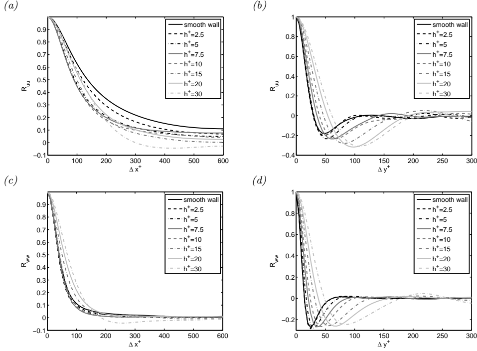
FIGURE 13. Two-point correlation measured at z^+ \approx 2h^+ ( z^+ = 5 in the reference case) for the streamwise (parts (a),(b)) and wall-normal (parts (c) and (d)) velocity component in streamwise and spanwise direction. Cases for a Gaussian shape function and a roughness factor \alpha = 1 .
