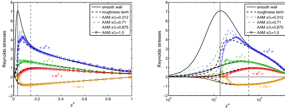
FIGURE 18. Direct comparison with AAM: Reynolds stresses normalised by u_{\tau_0}^2 . (a) in outer coordinates, (b) in inner coordinates. The thin black continuous vertical line indicates the height of the roughness elements. The thin black dashed vertical line indicates the extent of the roughness sublayer as estimated by AAM.
