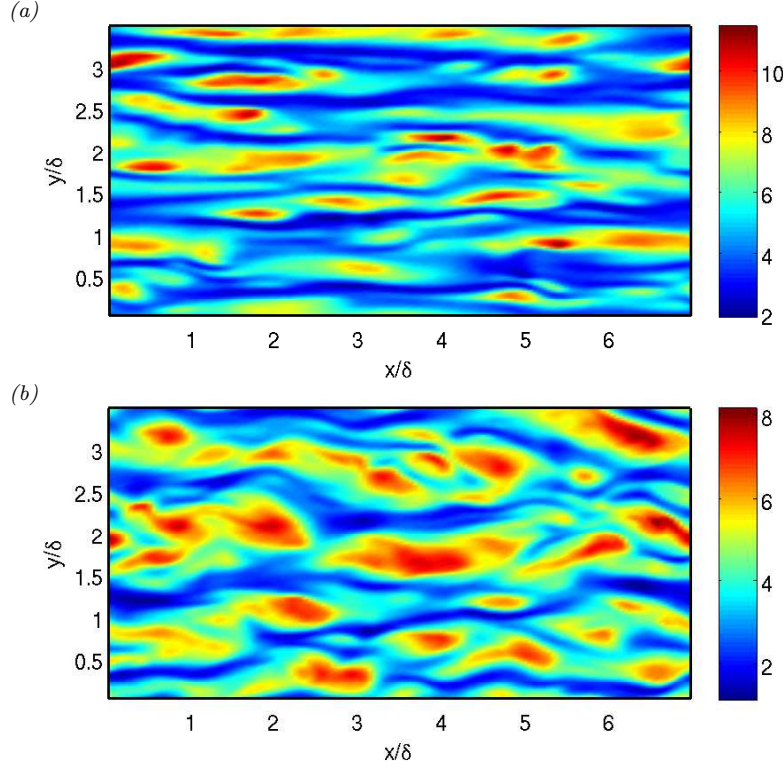
FIGURE 14. Contours of u for (a) smooth wall reference case at z^+ = 5 , (b) for case using a Gaussian shape function, \alpha = 1 , h^+ = 10 at z^+ = 20 . For the rough case a higher distance from the wall has been chosen in order to illustrate the flow ‘above’ the roughnesses, i.e. at z^+ = 2h^+ .
