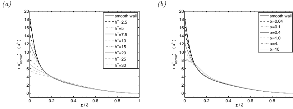
FIGURE 7. Velocity defect profile across the channel using a Gaussian shape function. Left: constant roughness factor \alpha = 1.0 and varying roughness height; right: varying roughness factor and constant roughness height parameter h^+ = 10 .
