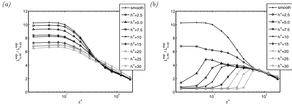
FIGURE 15. Ratio of streamwise to spanwise correlation length of streamwise velocity component. (a) \alpha = 0.1 , (b) \alpha = 10 ; Gaussian shape function.
