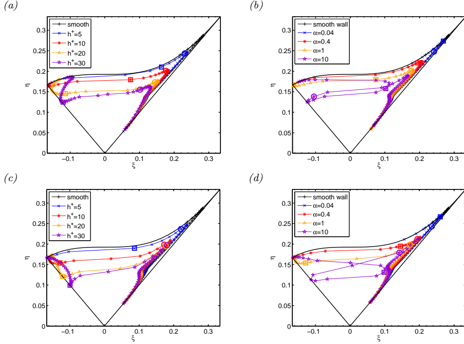
FIGURE 11. The anisotropy invariant map for the Reynolds stress anisotropy tensor. The black lines outline the Lumley triangle. (a), (b): cases for the Gaussian shape function. (c), (d): cases using the box shape function. (a), (c): results for different height parameters using \alpha = 1 ; (b), (d): results for different roughness factors using a constant roughness height of h^+ = 10 . The squares and circles indicate the data points obtained at distances from the wall equal to z^+ \approx h^+ and z^+ \approx 2h^+ .
