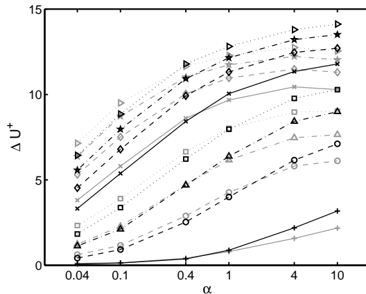
FIGURE 4. Roughness function plotted versus roughness factor for different values of the roughness height parameter (+: h^+ = 2.5 , \circ : h^+ = 5 , \triangle : h^+ = 7.5 , \square : h^+ = 10 , \times : h^+ = 15 , \diamond : h^+ = 20 , \star : h^+ = 25 , \triangleright : h^+ = 30 ); black symbols / lines: Gaussian shape function, grey symbols / lines: box shape function.
