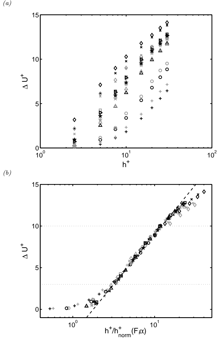
FIGURE 3. (a) Roughness function for different roughness factors and shape functions plotted versus roughness height parameter: for the Gaussian (black symbols) and box profile (grey symbols) results are shown for six different roughness factors (+: \alpha = 0.04 , ○: \alpha = 0.1 , △: \alpha = 0.4 , □: \alpha = 1. , ×: \alpha = 4 , ◇: \alpha = 10 ) and different shape functions. For the four remaining shape functions results are shown for \alpha = 1 : triangular profile (black ▷), parabolic profile (grey ▷) exponentially decaying profile (black ★), orbital profile (grey ★). (b) Roughness function plotted versus rescaled height parameter; legend for symbols as in part (a) of this figure. The dashed line shows the best fit (see eqn. 4.2) in the interval 3 \leq \Delta U^+ \leq 10 .
