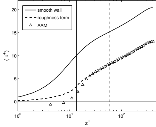
FIGURE 17. Direct comparison with AAM: mean streamwise velocity profile. The thin black continuous vertical line indicates the height of the roughness elements. The thin black dashed vertical line indicates the extent of the roughness sublayer as estimated by AAM.
