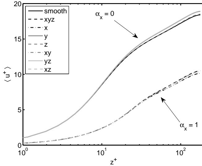
FIGURE 2. Mean streamwise velocity profile for different roughness factor \alpha_i combinations in the roughness force term. A Gaussian shape function has been used. The legend refers to the second column of table 1. The lower group of curves consists of cases including the streamwise component of the roughness term ( \alpha_x = 1 ), whereas for the upper group of curves \alpha_x = 0 .
