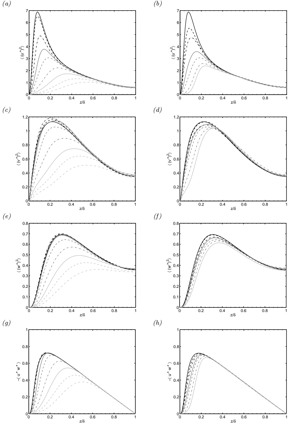
FIGURE 9. Profiles of Reynolds stresses across channel. (a) and (b): streamwise normal stress; (c) and (d): spanwise normal stress; (e) and (f): wall-normal stress; (g) and (h): shear stress. (a), (c), (e), (g): constant roughness factor \alpha = 1.0 and varying roughness height ( h^+ = 2.5, 5, 7.5, 10, 15, 20, 25, 30 ), line styles as in figure 6 (a). (b), (d), (f), (h): constant roughness height h^+ = 10 and varying roughness factor ( \alpha = 0.04, 0.1, 0.4, 1, 4, 10 ), line styles as in figure 6 (b). In all cases a Gaussian shape function as been used.
