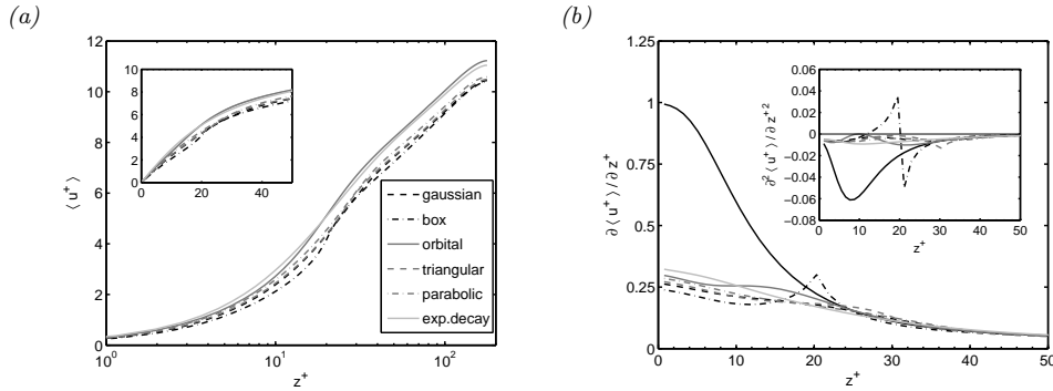
FIGURE 8. (a): Mean streamwise velocity profile across the channel for different shape functions (inset in linear scales). (b): 1st and 2nd (inset) derivatives of mean streamwise velocity profile. The roughness factor is \alpha = 1 , roughness height parameter h^+ = 10 . The legend of (a) applies also to (b), the black continuous line in (b) shows the smooth-wall reference case.
