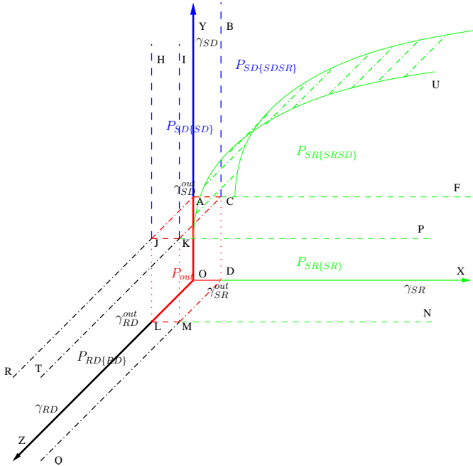
Fig. 3. The transmission activation probability space (TAPS) is divided by the outage SNR-thresholds into 8 regions. P_{out} is the outage probability of the system, while P_{SR}\{SR\} , P_{RD}\{RD\} and P_{SD}\{SD\} represent the probability that only the SN-RN, the RN-DN or the SN-DN channel is available, respectively.
