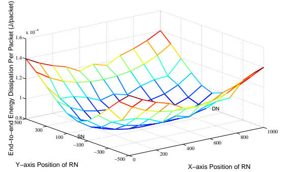
Fig. 7. Average normalized end-to-end energy dissipation vs the RN position. The results are theoretical analysis with assuming of infinity buffer size.
