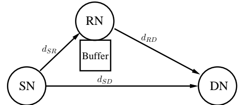
Fig. 1. System model for a buffer-aided three-node network, where SN sends messages to DN via RN, directly or indirectly.
