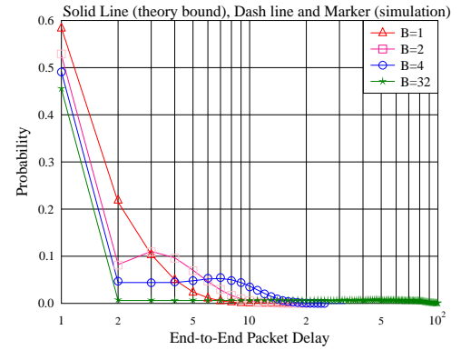
Fig. 9. The distribution of the packet delay evaluated from Section V, when the RN is at the position of (400, 400). The buffer size ranges from 1 to 32.
