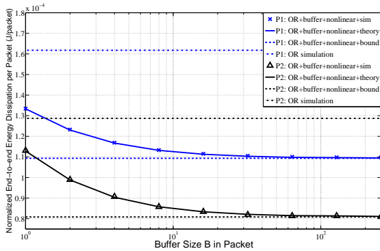
Fig. 5. Average normalized end-to-end energy dissipation per packet as defined in Section III-B when the RN is at the position of (400, 400) and the pathloss factor is \alpha = 2 . The theoretical curve was evaluated from (36).
