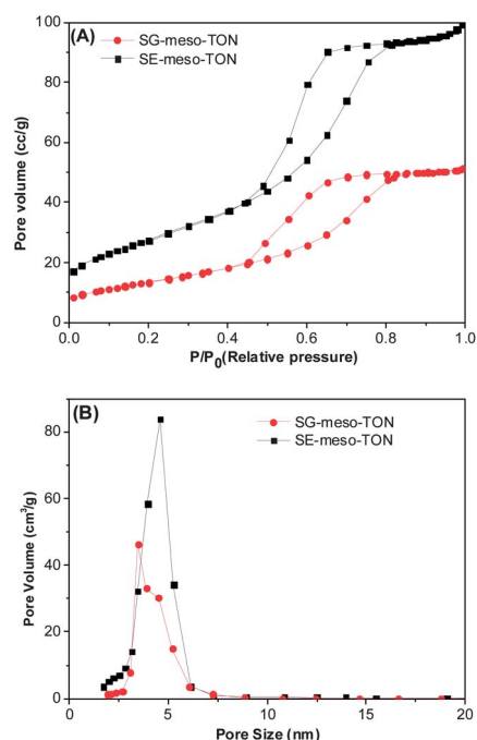
Fig. 3 N 2 adsorption–desorption isotherm (A) and pore size distribution (B) of the meso-TON samples calcined at 450 °C.
