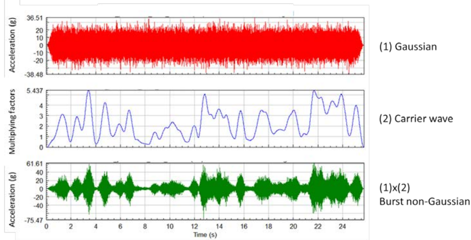
Figure 2: Construction of a burst non-Gaussian signal
