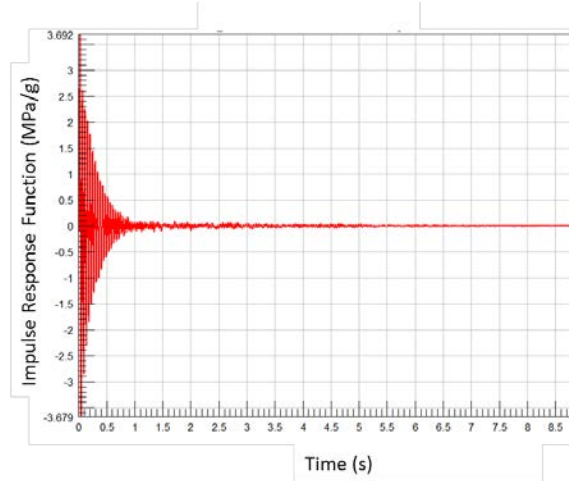
Figure 13: Impulse response function obtained from stress FRF at a critical node (3100).
