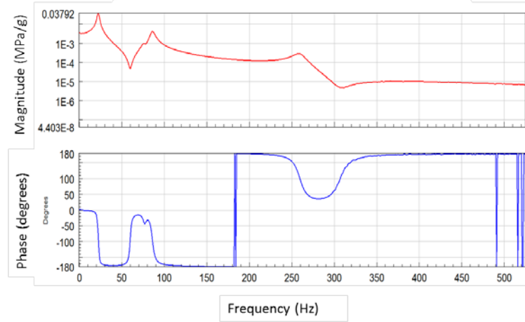
Figure 7: Stress FRF obtained at a critical node (3100).
