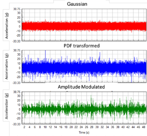
Figure 5: The excitation signals generated: Gaussian (red), steady non-Gaussian using PDF transform method (blue) and burst non-Gaussian using amplitude modulation method (green).
