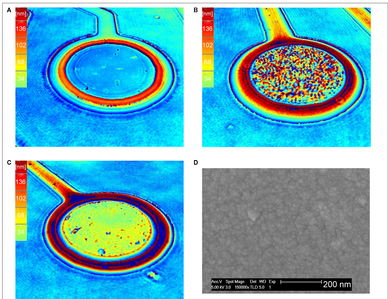
FIGURE 5 | The surface roughness of MEAs, before and after IrOx activation, studied by digital holographic microscopy ( A–C ) and scanning electron microscopy ( D ). The first technique reveals a substantial difference in the vertical nanometer scale surface roughness following IrOx activation ( B ), compared to electrode surface before activation ( A ). ( B ) Shows an
