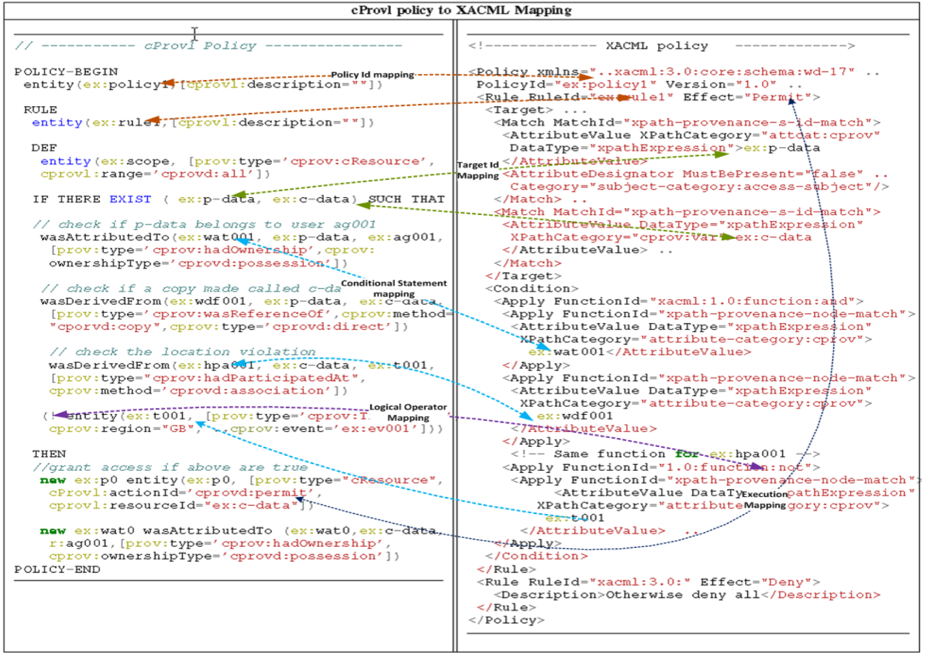
Fig. 4: cProv to XACML - Scenario Policy One
