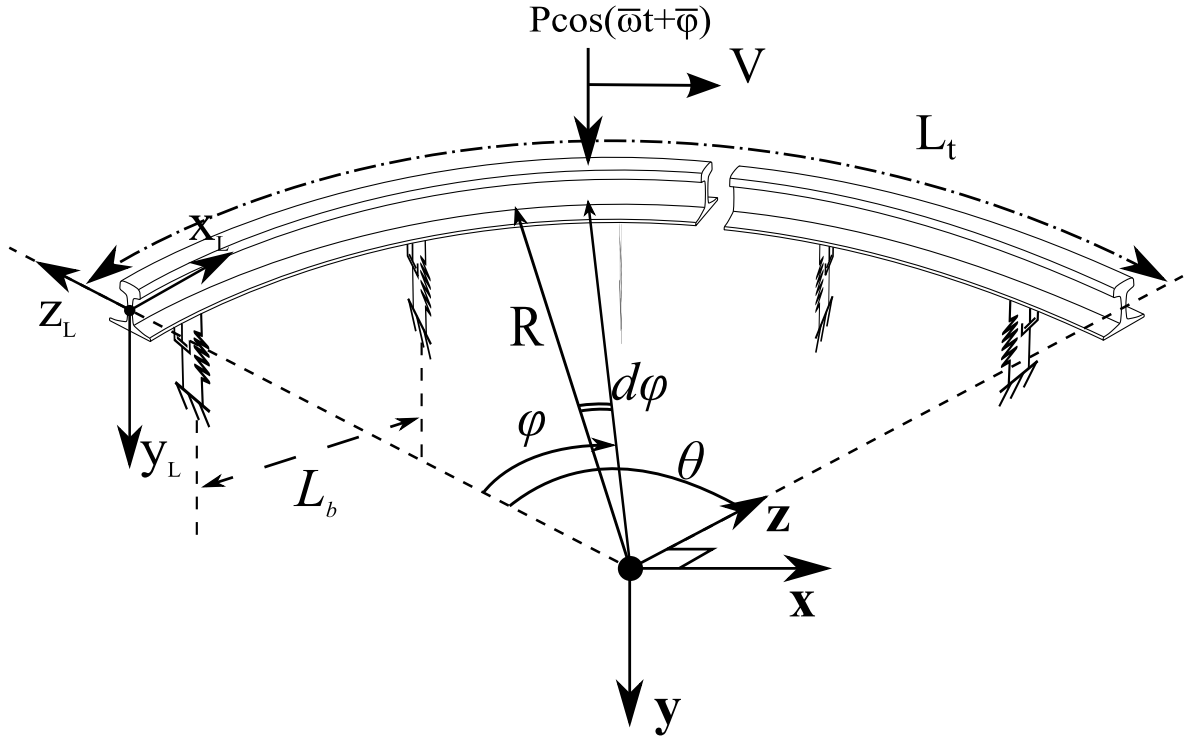
Figure 1: Curved beam on elastic foundation
