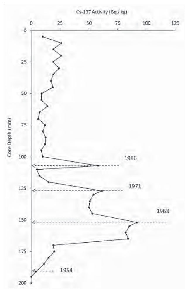
Fig. 3 Depositional fallout history of ^{137}\text{Cs} , as recorded in a short core of sediment obtained from Lake Shudu
