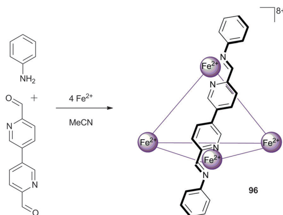
Scheme 10 The construction of Nitschke's \text{M}_4\text{L}_6 cages with reconfigurable exterior.
