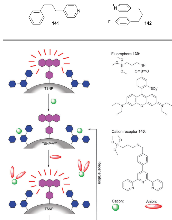
Scheme 17 Design concept of the anion quencher displacement assay (QDA) involving terpyridine-sulforhodamine functionalised nanoparticle (TSNP) and a metal ion quencher, along with the structure of fluorescent dye 139 (magenta) and cation receptor 140 (blue).
