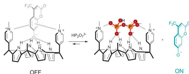
Scheme 3 Proposed Fluorescent Dye Displacement Assay (FDDA) detection of pyrophosphate anion by 45 .
