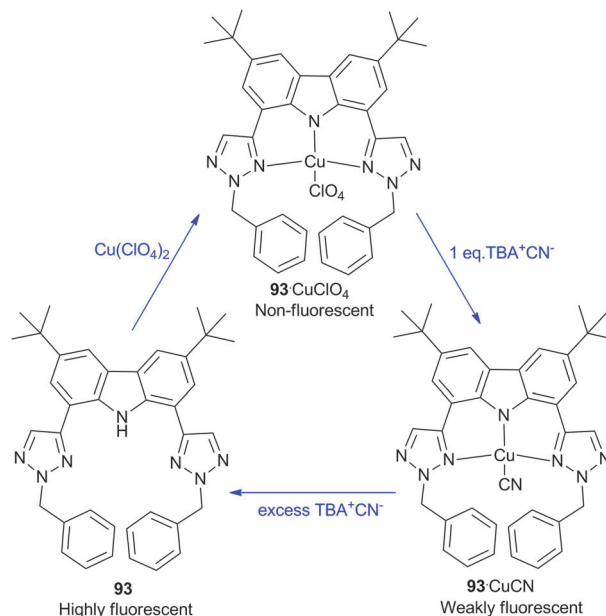
Scheme 9 The proposed mechanism of \text{CN}^- sensing by the 93 –Cu(II) complex.
