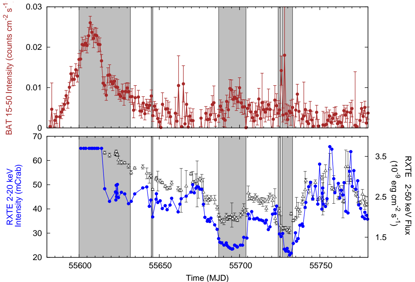
FIG. 1.— Upper Panel: Swift /BAT light curve. Lower Panel: Circles: RXTE Crab normalized 2-20 keV intensity. RXTE values are averaged per observation, background subtracted and dead-time corrected. Triangles: RXTE 2-50 keV flux. RXTE observations between day 55601 and 55615 are affected by the nearby source GX 349+2 (Sco X-2); the intensity during this period was arbitrarily fixed to 65 mCrab and no X-ray flux is reported. Shaded areas mark quiet periods (see text).
