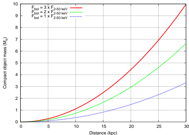
FIG. 5.— Mass of the compact object versus distance to the binary system assuming IGR J17091-3624 is emitting at Eddington. The three curves correspond to different (1, 2 and 3) correction factors between the 2-50 keV and the bolometric flux.
