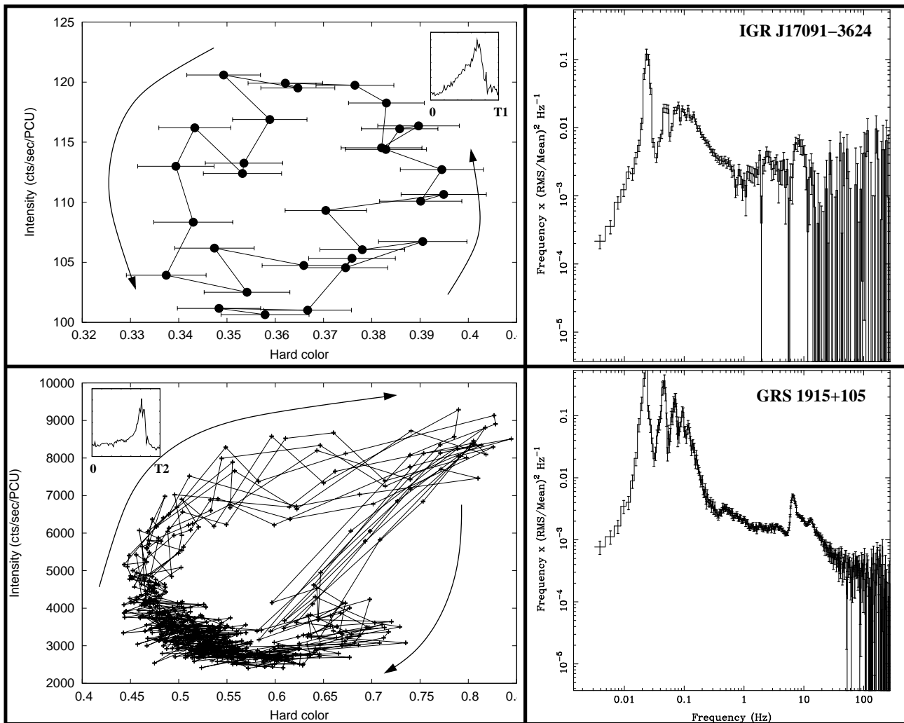
FIG. 4.— Left panels show the hardness-intensity diagram for flares observed during the \rho variability class in IGR J17091-3624 (top; ObsID 96420-01-04-03) and GRS 1915+105 (bottom; ObsID 96378-01-01-00) occurring at an average period of T_1=70.96 seconds and T_2=63.72 seconds, respectively. Arrows mark the time evolution. Inset shows representative flares. Light curves and colors are estimated from 1 sec averages. Intensity is the count rate in the 2-60 keV range (absolute channels 0-240) and hard color is the 6.5–15.0 keV / 2–6.5 keV count rate ratio (channels 15-35 and 0-14, respectively). Right panels show representative power spectra from averages of 512 sec segments during the \rho variability class for IGR J17091-364 (top, ObsID:96420-01-05-000, MJD 55647.9) and for GRS 1915+105 (bottom, ObsID:40703-01-07-00, MJD 51235.3).
