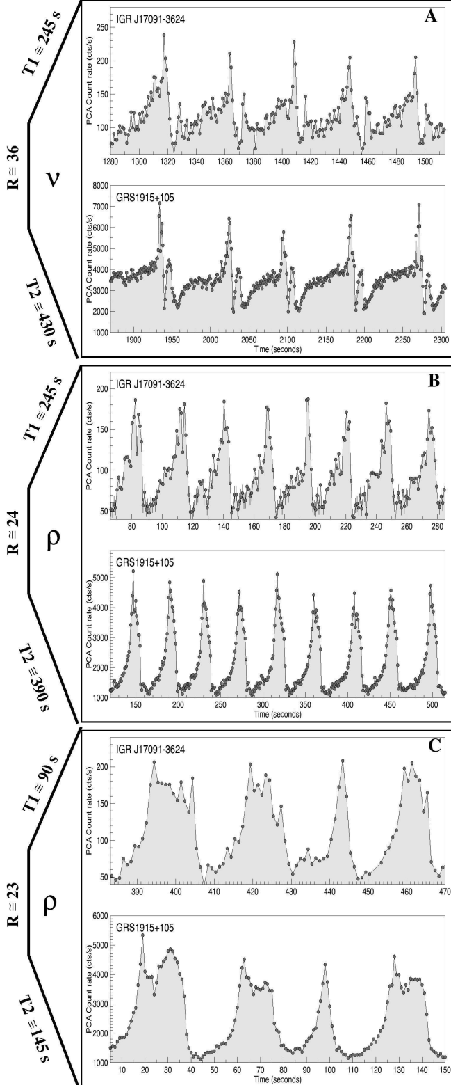
FIG. 2.— The upper and lower panels of each frame show a light curve of IGR J17091–3624 and GRS 1915+105, respectively. Count rates are given in 1 s bins, per PCU, 2–60 keV and background subtracted. The IGR J17091–3624 A–C intervals last T_1 seconds and come from observations 96420-01-05-00, -06-00 and -07-01, respectively. For GRS 1915+105 they last T_2 seconds and come from observations 10408-01-40-00, 20402-01-34-00 and 93701-01-02-01, respectively. R \equiv MIN_{GRS\ 1915+105}/MIN_{IGR\ J17091-3624} , where MIN is an average count rate during minima in the above light curve and is given for each frame as an order of magnitude estimate of the flux ratio. Greek letters on the side indicate variability the class.
