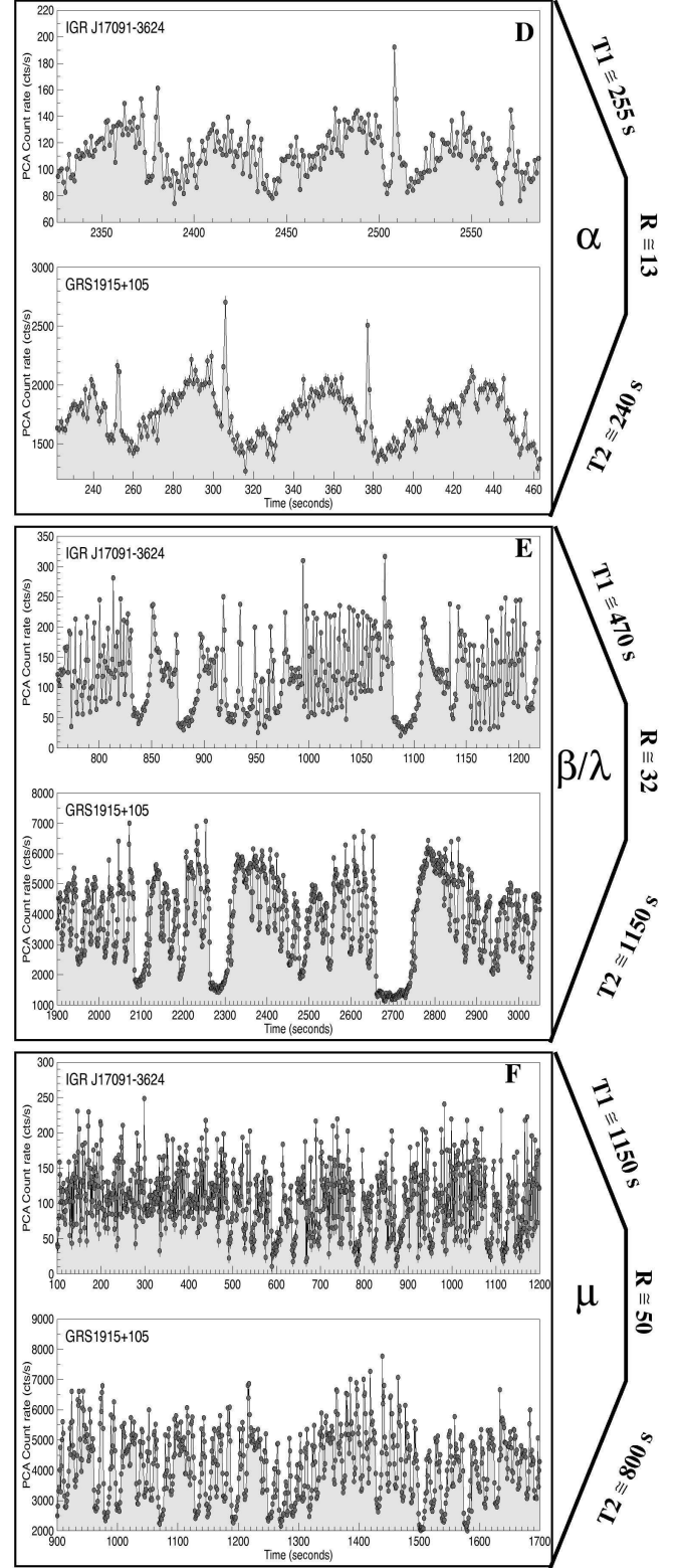
FIG. 3.— Similar to Figure 2. The IGR J17091–3624 D–F intervals come from observations 96420-04-03, -08-03 and -09-06, respectively. For GRS 1915+105 they come from observations 20187-02-01-00, 95701-01-31-00 and 10258-01-10-00, respectively.
