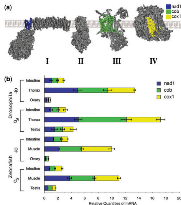
Fig. 1. —Relative quantities of mitochondrial mRNA measured for three key protein subunits of the mitochondrial respiratory chain. (a) A schematic representation of the respiratory electron transport chain of the mitochondrial inner membrane. The protein subunits highlighted in blue, green, and yellow represent the products of the mitochondrial genes nad1 , cob , and cox1 , respectively. Structures are surface models drawn using PyMol (Schrodinger 2010) from Protein Data Bank (PDB) atomic coordinate files with the following accession numbers: respiratory complex I (NADH-ubiquinone oxidoreductase), 3M9S; respiratory complex II (succinate dehydrogenase), 1Z0Y; respiratory complex III (the cytochrome b-c 1 complex), 1QCR; complex IV (cytochrome c oxidase), 1V54. (b) Respiratory electron transport gene expression profile. Quantities are shown for mitochondrial mRNA expressed in different tissues of male and female individuals of D. melanogaster and D. rerio . The color coding is the same as that used in (a): blue, nad1 ; green, cob ; yellow, cox1 . Error bars indicate standard error of the mean (SEM). P \leq 0.05 . See also supplementary tables S1 and S2, Supplementary Material online .
