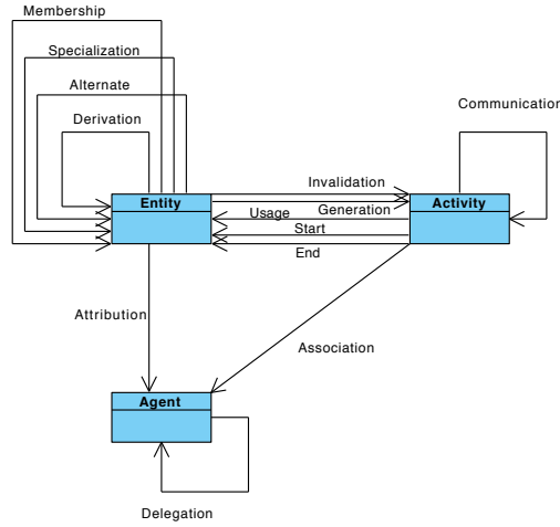
Fig. 1. PROV-DM UML Classes and Associations (simplified view)
