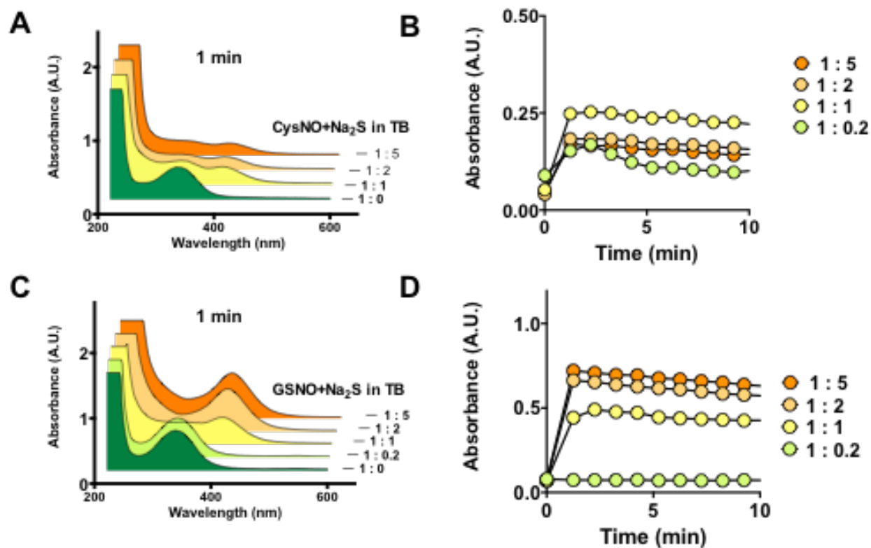
Figure S2: Formation of SSNO - from CysNO and GSNO in aqueous conditions. Reaction of CysNO (1 mM) (A,B) or GSNO (C,D) with different concentrations of Na 2 S (0.2; 1; 2; or 5 mM) and in TRIS buffer 1M (TB) at pH 7.4. (A,C) UV-visible spectra of the different concentration ratios taken after 1 min of incubation. Green spectra, starting spectrum of CysNO (A) or GSNO (C). (B,D) Kinetics of formation of SSNO - ( \lambda_{\text{max}} 412 nm) from CysNO (B) and GSNO (D).
