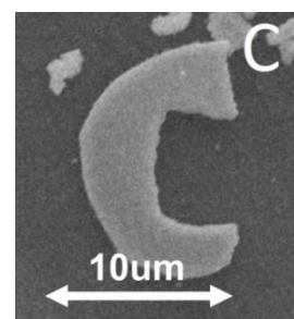
Shaped printing of \text{Bi}_2\text{Te}_3
