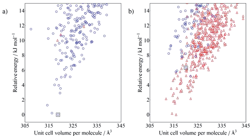
Fig. 4 Calculated crystal energy landscapes of (a) 2\text{NO}_2 \cdot 2\text{NO}_2 and (b) 4\text{Me}_4\text{Me} . Each point corresponds to a distinct crystal structure, whose total energy is reported relative to the lowest energy predicted structure. The open blue circles are structures generated by the molecular conformer that is closest to the observed conformer, and open red triangles are from the other conformers. The prediction that matches the observed structure is indicated by an open square.
