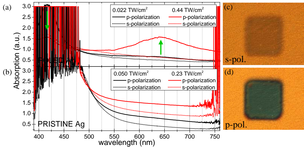
Fig.2. Absorption spectra of (a) poled areas modified with 2.2 \times 10^{10} W/cm 2 and 4.4 \times 10^{11} W/cm 2 laser pulse intensities and (b) pristine areas modified with 5.0 \times 10^{10} W/cm 2 and 2.3 \times 10^{11} W/cm 2 , spectra were collected both for s- and p-polarized excitation. (c,d) Images of the poled area modified with the highest energy, for s- and p-polarized illumination, respectively. Green arrows indicate the direction of movement of spectra after the modification.
