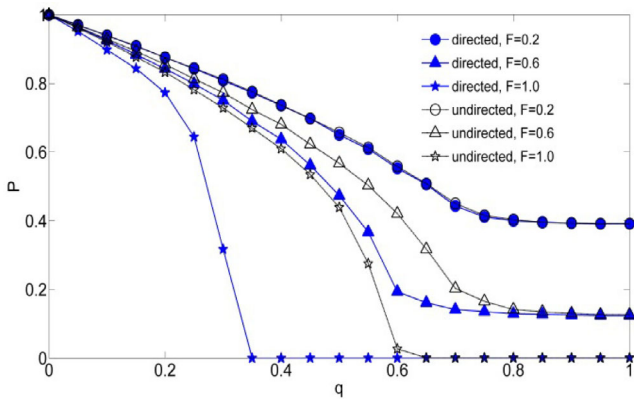
Fig. 8. Relative size of giant component P as a function of q (the size of the attack on network A ), where \mathcal{K}^{A,B} = \mathcal{K}^{B,A} = 2 , and \mathcal{F}^{A,B} = \mathcal{F}^{B,A} = F are varied.
