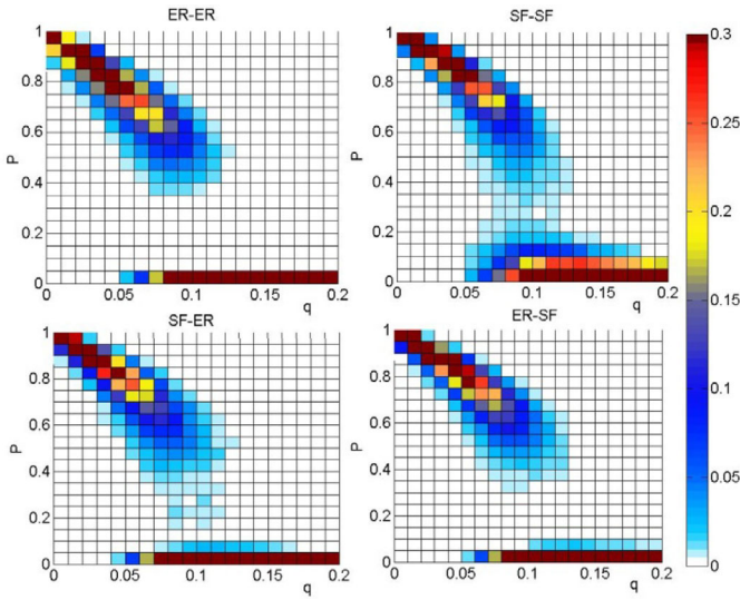
Fig. 11. Impact of network topologies. Frequency of relative size of giant component P is plotted as a function of q and P . Dependencies are set with \mathcal{D}^{A,B} = \mathcal{D}^{B,A} = 1 , \mathcal{F}^{A,B} = \mathcal{F}^{B,A} = 0.8 and \mathcal{K}^{A,B} = \mathcal{K}^{B,A} = 1 .
