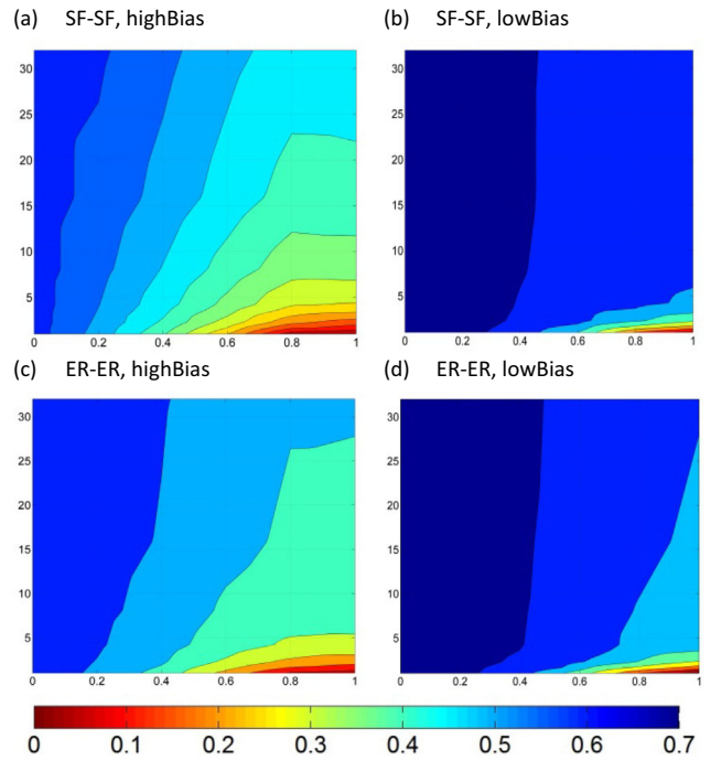
Fig. 12. Results for systems under lowBias and highBias attacks. Aggregate performance IP is plotted as a function of \mathcal{K}^{A,B} = \mathcal{K}^{B,A} = K (vertical axis) and \mathcal{F}^{A,B} = \mathcal{F}^{B,A} = F (horizontal axis), under dependency setting of \mathcal{D}^{A,B} = \mathcal{D}^{B,A} = 1 .
