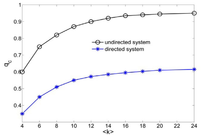
Fig. 10. Impact of network node degree. Failure threshold q_c is plotted as a function of K_0^A = K_0^B = \langle k \rangle for systems under the interdependency setting of \mathcal{F}^{A,B} = \mathcal{F}^{B,A} = 1.0 and \mathcal{K}^{A,B} = \mathcal{K}^{B,A} = 2 .
