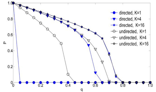
Fig. 7. Relative size of giant component P as a function of q (the size of the attack on network A ), where \mathcal{F}^{A,B} = \mathcal{F}^{B,A} = 1.0 , and \mathcal{K}^{A,B} = \mathcal{K}^{B,A} = K are varied.
