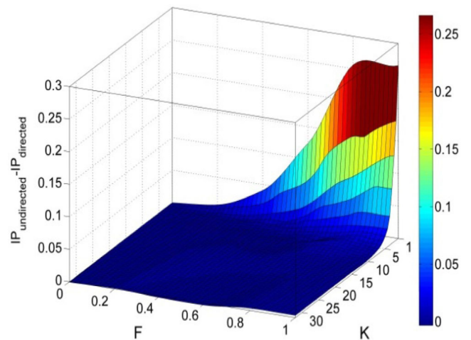
Fig. 4. Difference between the aggregate performance ( IP_{undirected} - IP_{directed} ) of undirected and directed systems when \mathcal{K}^{A,B} = \mathcal{K}^{B,A} = K and \mathcal{F}^{A,B} = \mathcal{F}^{B,A} = F are varied.
