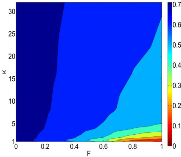
Fig. 3. Aggregated system performance IP of a directed interdependent system with \mathcal{K}^{A,B} = \mathcal{K}^{B,A} = K and \mathcal{F}^{A,B} = \mathcal{F}^{B,A} = F .
