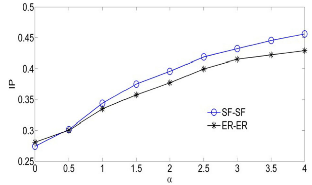
Fig. 14. Performance improvement when high degree nodes are hardened. Aggregate performance, IP , is plotted as function of \alpha as specified in equation (4). Both SF-SF and ER-ER systems have dependency setting \mathcal{D}^{A,B} = \mathcal{D}^{B,A} = 1 , \mathcal{F}^{A,B} = \mathcal{F}^{B,A} = 1.0 and \mathcal{K}^{A,B} = \mathcal{K}^{B,A} = 2 .
