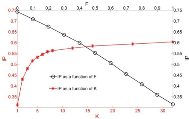
Fig. 6. Aggregate performance IP as a function of K ( \mathcal{K}^{B,A} = \mathcal{K}^{B,A} = K , \mathcal{F}^{A,B} = \mathcal{F}^{B,A} = 1 and \mathcal{D}^{A,B} = \mathcal{D}^{B,A} = 0 ), and IP as a function of F ( \mathcal{F}^{A,B} = \mathcal{F}^{B,A} = F , \mathcal{K}^{A,B} = \mathcal{K}^{B,A} = 1 and \mathcal{D}^{A,B} = \mathcal{D}^{B,A} = 0 ).
