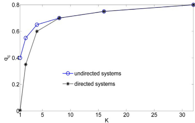
Fig. 5. Failure threshold, q_c , as a function of \mathcal{K}^{A,B} = \mathcal{K}^{B,A} = K when \mathcal{F}^{A,B} = \mathcal{F}^{B,A} = 1.0 .
