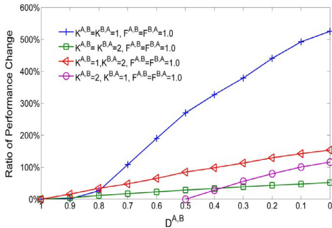
Fig. 13. Reducing vulnerability: ratio of performance change in term of aggregate performance IP , when the proportion, \mathcal{D}^{A,B} , of directed dependencies decreases in an interdependent system.
