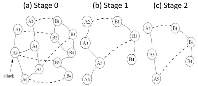
Fig. 2. Cascading failure process of an interdependent system. The initial system, shown in (a), has a set of nodes in network A and B , labelled \{A_1, A_2, \dots\} and \{B_1, B_2, \dots\} , respectively. An intra-link is represented as a solid line, and an inter-link is represented as a dashed line. At Stage 0, node A_4 is disabled/attacked. When A_4 fails, all links connected to A_4 fail. This disconnects A_1 from the largest component of network A , and therefore A_1 fails. The failure of A_4 and A_1 triggers the failure of B_5 (supported by A_4 ) and B_2 (supported by A_1 ). The failure of B_5 disconnects B_6 from the largest component of network B , hence B_6 fails. This leads to the system configuration shown in (b). The failure of B_6 leads to the failure of A_6 , before the system eventually stabilises in the configuration shown in (c).
