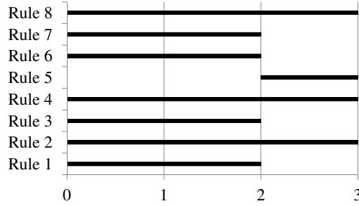
Figure 2: Rule Schedules
