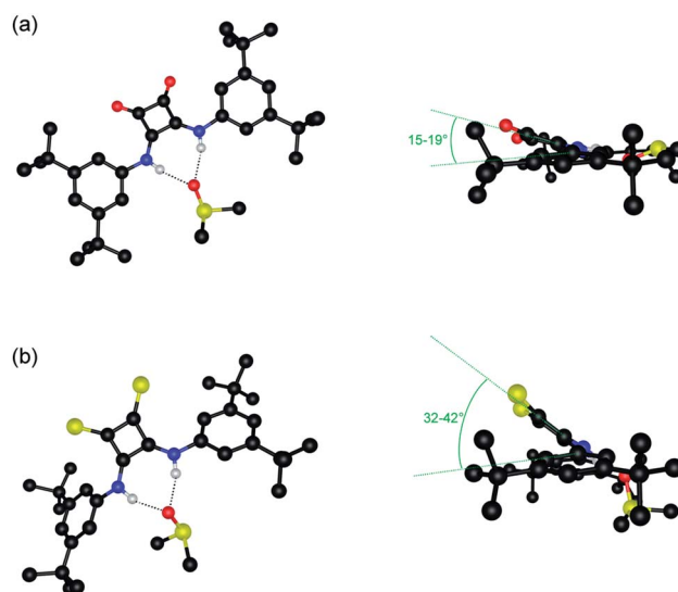
Fig. 1 Front and side views of the X-ray crystal structure of 4 ·DMSO (a) and 8 ·DMSO (b). Ligands and DMSO molecules are shown in ball-and-stick. Non-interacting hydrogen atoms and non-interacting DMSO molecules are omitted for clarity. Hydrogen bonds are represented by dashed lines and atoms are colour coded as follows: C (black), H (white), F (green), N (blue), S (yellow) and O (red). Relevant torsion angles are given in green.
