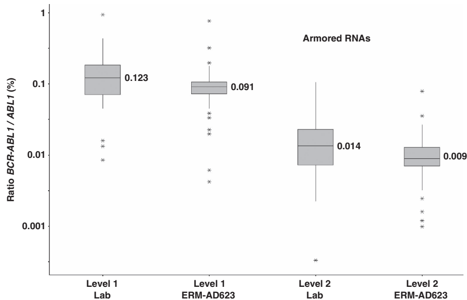
Figure 3. Comparison of measured \% \text{BCR-ABL1/ABL1} ratio between laboratory calibrators (Lab) and ERM-AD623 for the aRNA mixtures. Data from all centres in the second suitability study that used ABL1 as a control gene and returned aRNA data are included; median values are indicated.
