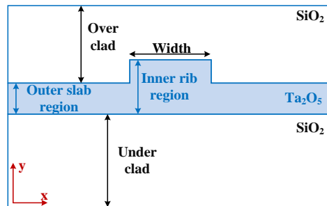
Figure 1. Cross-section of etched rib waveguide design
