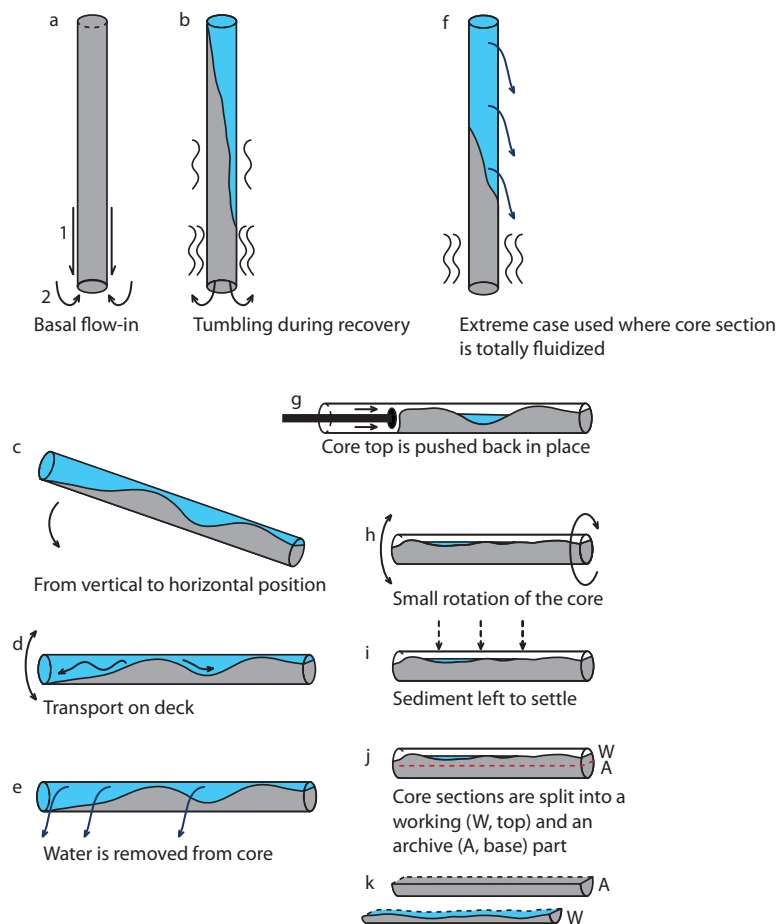
Figure 9. Possible disturbances in sandy to gravelly cores retrieved by APC. (a) Sudden release of the core liner into the sediment (1); sucking in of loose clasts at the bottom of the core liner during retrieval, creating basal flow-in (2; see Figure 4); (b) tumbling on the core barrel and vertical accelerations during recovery; release of small amount of loose sediments through the core catcher; (c) transfer of the core liner to a horizontal position on deck; (d) loose clasts flush back and forth during transport and lying down on deck (cat walk); (e) the core liner is drilled at many places to release excessive pore pressure. Small volumes of fines are lost; (f) rare case when abundant water is in the core. The core liner has to be put in vertical position to release exceeding seawater; (g) loose patches of sediments at the top of the core liner are pushed together to make a coherent core volume, any voids are therefore lost; (h) the core liner is cut in \sim 1.50 m long sections, which are eventually rotated to put the archive-half on the lower part of the cylinder; (i) sediment settles for 3 h to reach ambient ship temperature; occasional shaking and tumbling when analyzed as whole core on two track systems; (j) the core liner is split lengthways, from base to top; (k) the working-half (W) is commonly much less voluminous than the archive-half (A), corresponding to fluid loss.
