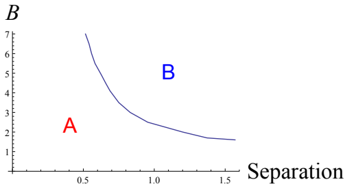
FIG. 4: Phase diagram of bi-layer D5s in AdS with one compact direction and an applied B field. Phase A is U-shaped configurations. In Phase B the probes separate and take up configurations similar to Fig 1.
