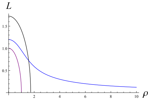
FIG. 1: The embedding of a single D5 brane for a massless quark in the AdS-soliton background is shown for r_0 = 1 . The dual of the compact space therefore closes off on the smaller circle shown - note the D5 brane embedding is regular avoiding this line. We also show the solution of (21) with the tension chosen so that the interval between the walls has radius R^2\pi/r_0 - the D5 embedding hits this cut off on the space.
