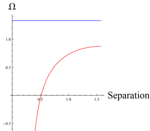
FIG. 3: The regularized energy of two D5s in the configuration of Fig 1 (which is independent of z ) and that of the U-shaped joined embedding against separation in z (which cannot exceed \pi/2 ). The U shaped configurations are always preferred.
