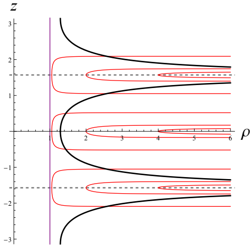
FIG. 2: U-shaped D5/ \bar{D}5 configurations in the AdS-soliton background. The space has circumference \pi in the z -direction - we repeat the space to show configurations wrapping both ways around the circle. Note that configurations which reach down to r_0 = 1 describe defects separated by \pi/2 in z . We also plot the solution of (21) with the tension chosen so that the interval between the walls is \pi - the probe configurations hit this boundary. If the figure is viewed as that for an interval between two mirrors then configurations corresponding to exciton condensation with the mirror partner exist if the probe lies within \pi/4 of the mirror.
