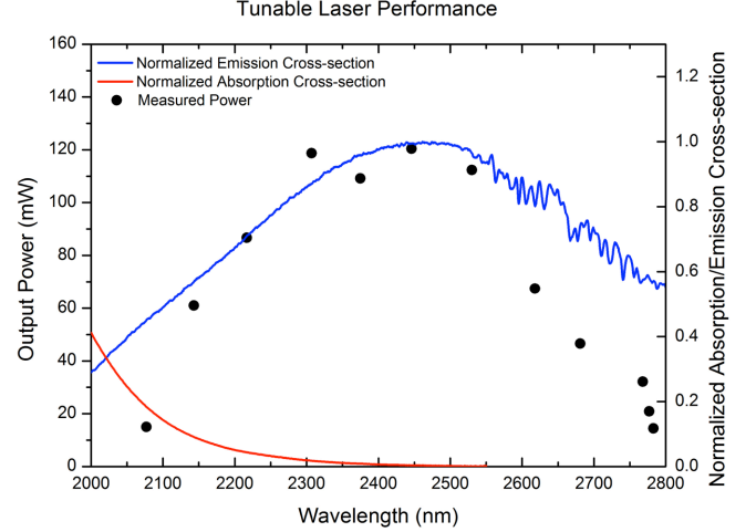
Fig. 2. Tunable Cr: ZnSe laser performance. Black dots represent measured output power at specific wavelengths. The blue and red line represent normalized emission and absorption cross-sections respectively for Cr:ZnSe.
