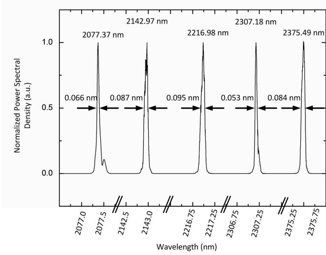
Fig. 3. Narrow linewidth spectra of the tunable Cr: ZnSe waveguide laser measured with a mid-infrared spectrum analyzer. A minimum linewidth of 0.053 nm is recorded at 2307 nm with all measured spectra demonstrating linewidths under 100 picometers FWHM.
