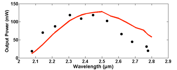
Fig. 4. Numerical model of tunable laser output and experimentally obtained data. Red line represents the theoretical model and black dots represent measured data points. No free fitting parameters have been used in the theoretical model.
