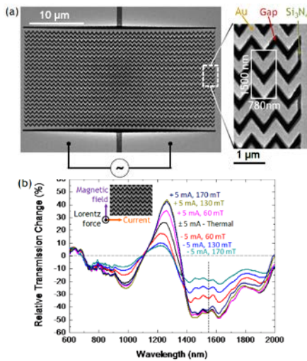
Figure 2. (a) Structure of the reconfigurable photonic metamaterial consisting of free-standing plasmonic zig-zag shaped bridges, where every second bridge is connected to electrical terminals on both ends, see close-up of the bridges ends. (b) Magnetic tuning of the reconfigurable photonic metamaterial. Relative transmission change as a function of applied device current and magnetic field.
