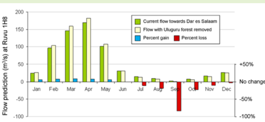
Figure 2. Broad-scale model (WatR) predicts that conversion of forest to cropland in Uluguru would result in reduced Ruvu River flow towards Dar es Salaam during the driest months of the year potentially leading to water shortages, whilst increasing peak flow during the wet season potentially leading to erosion and flooding
