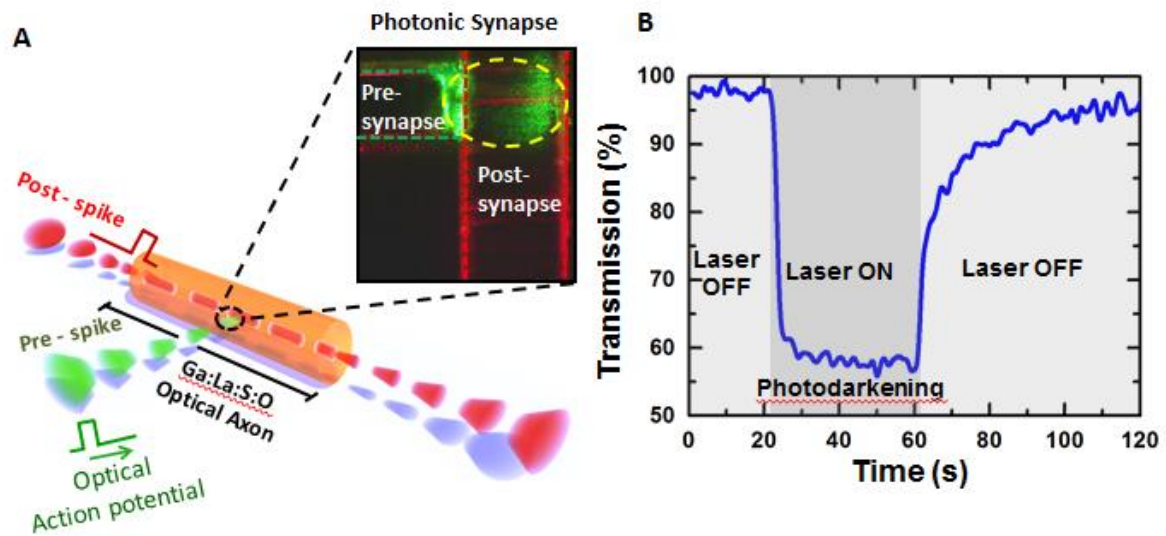
Figure 2: (A) The optical neuron transmits information through optical signals (laser pulses) that propagate along a gallium lanthanum oxysulphide fiber, and use photodarkening as a result of sub-bandgap light exposure at the photonic synapse (inset) to induce inhibitory and excitatory action potentials in the post-synaptic axon. (B) Photodarkening occurring upon exposure of the GLSO microfiber to sub-bandgap excitation ( \lambda=532 nm, I=130 mW) within the period 20 to 60 s reduces transmission of guided light ( \lambda=650 nm, I=10 mW) by \sim 40\% .
