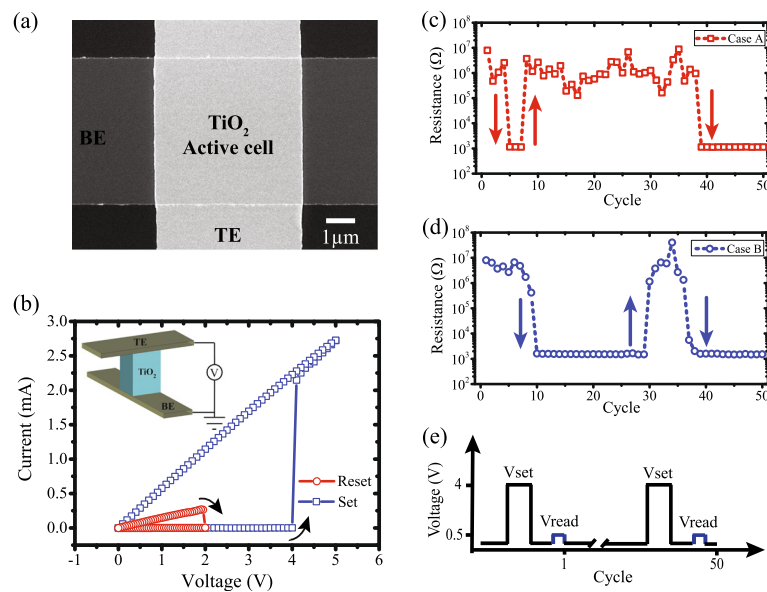
Figure 1 Measured features of \text{TiO}_2 -based ReRAM devices. (a) SEM image of a crossbar-type prototype based on \text{TiO}_2 cell with an active area of 5 \times 5 \mu\text{m}^2 . (b) Measured I - V characteristics showing a typical unipolar switching signature. Inset: schematic view of the measured cell. (c, d) Resistance evolution results of two practical devices with identical initial resistive states at room temperature. (e) Pulse-induced programming and evaluating scheme, where V_{\text{set}} and V_{\text{read}} represent resistance programming and evaluating pulses, respectively.
