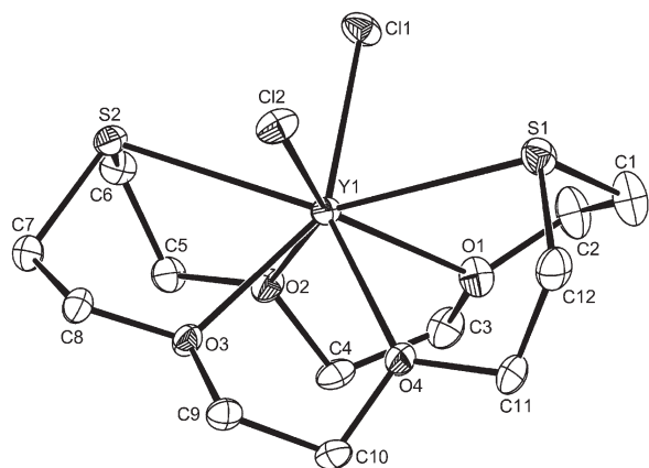
Fig. 5 The structure of the cation in [\text{YCl}_2([\text{18}]ane\text{O}_4\text{S}_2)][\text{FeCl}_4] showing the atom labelling scheme. The displacement ellipsoids are drawn at the 50% probability level and H atoms are omitted for clarity. Selected bond lengths ( \text{\AA} ) and angles ( ^\circ ): \text{Y1-O2} = 2.3652(17) , \text{Y1-O4} = 2.4012(17) , \text{Y1-O3} = 2.4703(17) , \text{Y1-O1} = 2.4911(18) , \text{Y1-Cl1} = 2.5682(8) , \text{Y1-Cl2} = 2.5914(7) , \text{Y1-S2} = 2.8955(8) , \text{Y1-S1} = 2.9162(8) , \text{O4-Y1-O} = 3.67.15(6) , \text{O2-Y1-O1} = 66.43(6) , \text{Cl1-Y1-Cl2} = 94.63(2) , \text{O2-Y1-S2} = 68.09(4) , \text{O3-Y1-S2} = 68.26(4) , \text{O4-Y1-S1} = 69.20(5) , \text{O1-Y1-S1} = 66.58(4) .
