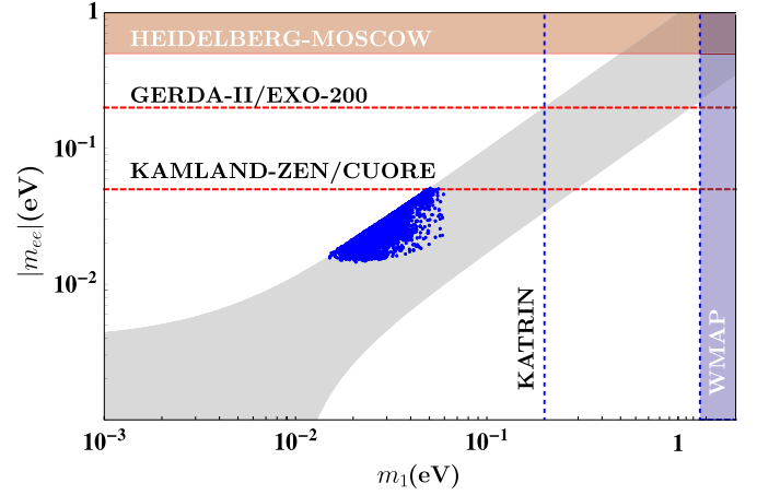
Fig. 1. Effective neutrino mass parameter m_{ee} as function of the lightest neutrino mass. The gray shaded regions correspond to the flavor-generic normal hierarchy neutrino spectra. The blue points correspond to the prediction of our A_4 model. For comparison we give the current and future sensitivities for m_{ee} [25,26] and m_\nu [27, 28], respectively. (For interpretation of the references to color in this figure legend, the reader is referred to the web version of this Letter.)
