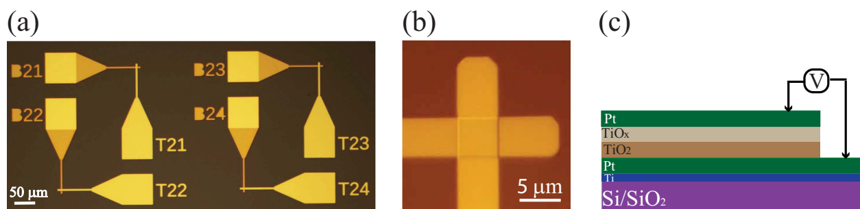
Figure 1 Optical microscope image, active area, and schematic of different devices. (a) Optical microscope image of a dense stand-alone device; (b) active area of a single 5 \times 5 \mu\text{m}^2 device; (c) schematic configuration of the Pt/TiO 2 /TiO x /Pt devices.
