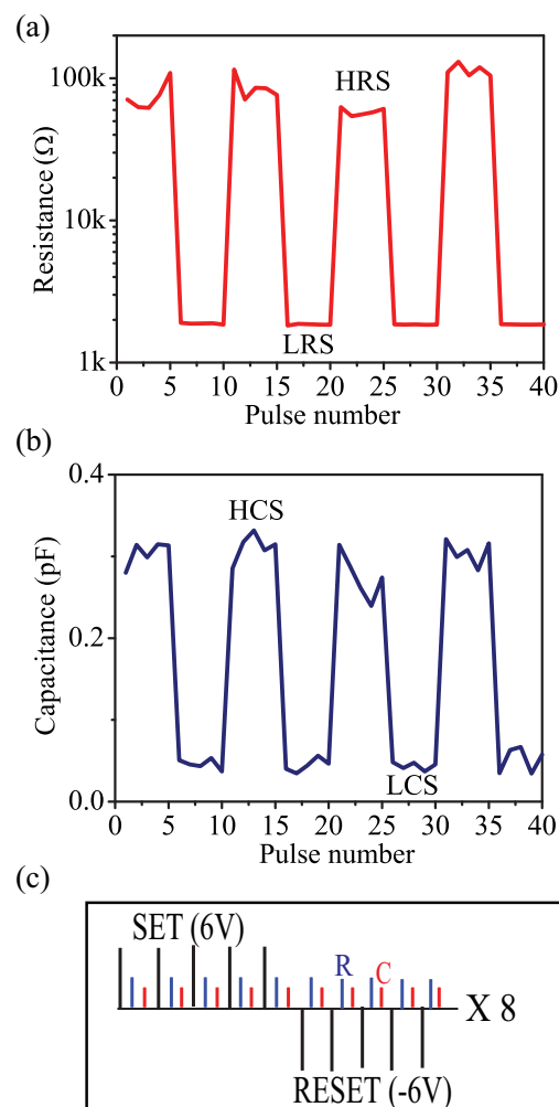
Figure 4 Concurrent capacitance/resistance modulation of TiO 2 -based solid-state devices. (a) Electrical pulse-induced resistance change, (b) electric pulse-induced capacitance change, (c) pulses sequences utilizing for concurrent resistive and capacitive state programming.
