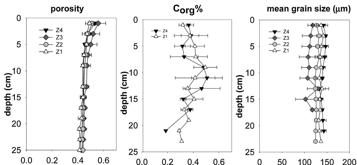
Fig. 5. Porosity, organic carbon content ( C_{org}\% ) and mean grain size of the upper 25 cm of the sediments in the experiment Zones 1 to 4. The horizontal bars are the variation of the parameters during the experiment at each site.
