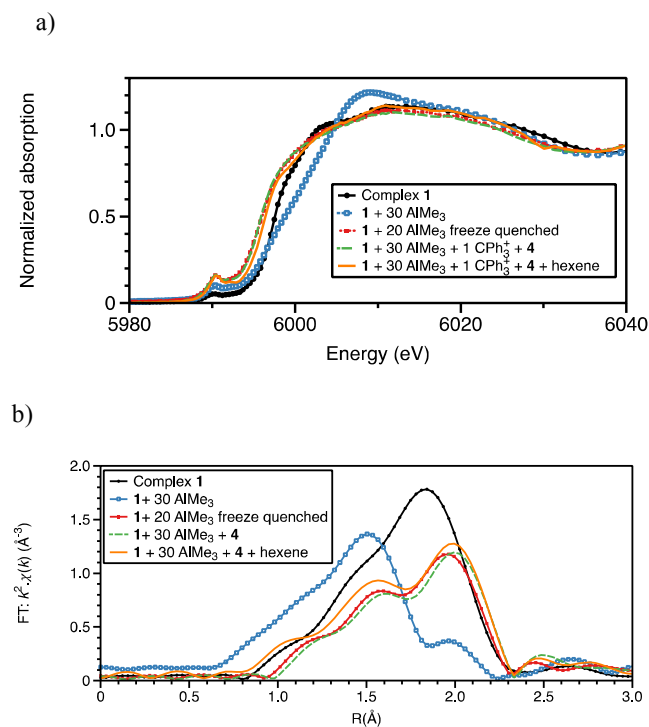
53 Figure 1. At the Cr K-edge: a) XANES and b) Fourier transforms 54 of k^2 -weighted EXAFS data for [\text{CrCl}_3\{\text{R-SN}(\text{H})\text{S-R}\}] 1 55 ( R=n -decyl) ( \bullet ) (5 mM in toluene) and reactions with \text{AlMe}_3 . 56 57 58 59 60
