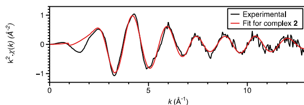
Figure 2. Cr K-edge k^2 -weighted EXAFS data for [\text{CrCl}_3\{\text{R-SN}(\text{H})\text{S-R}\}] 1 ( R=n -decyl) and \text{AlMe}_3 in toluene, freeze quenched.
