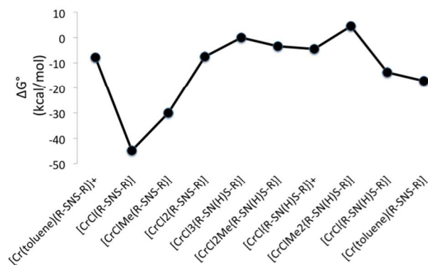
Figure 4 Calculated \Delta G^\circ (kcal/mol) of reaction steps from [\text{CrCl}_3\{\text{R-SN}(\text{H})\text{S-R}\}] 1 (R=Me) per Cr atom relative 1 , \text{Al}_2\text{Me}_6 and toluene.
