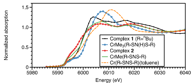
Figure 3. Calculations of the Cr K-edge XANES for 1 (R= n Bu) and possible reaction products.
