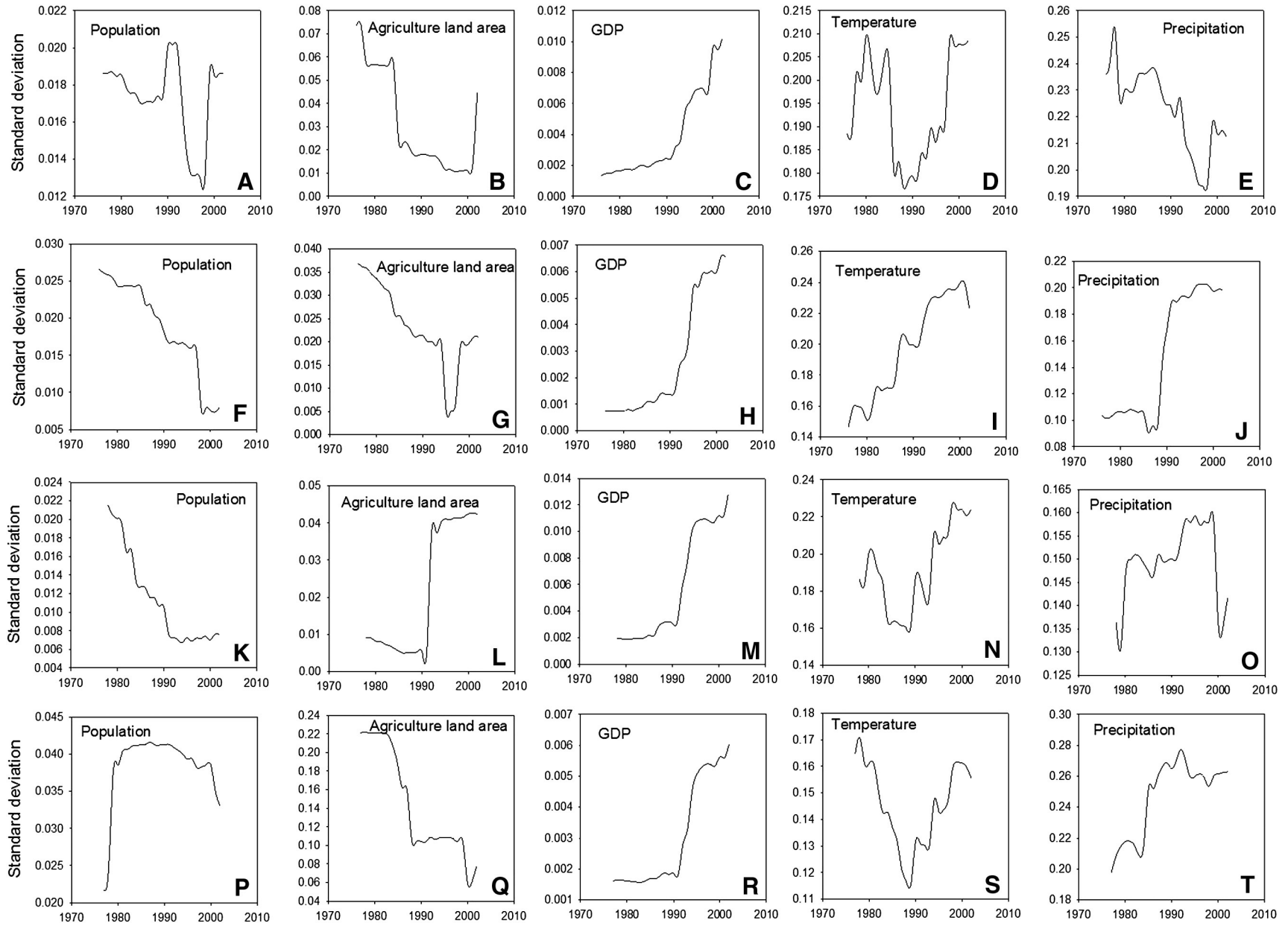
Fig. A.7. Variance (standard deviation) of possible individual drivers in each region: A–E, Huangmei; F–J, Shucheng; K–O, Wujiang; and P–T, Yangtze tidal zone. The standard deviation is calculated for a moving window (half time series) of residuals after detrending the original data.
