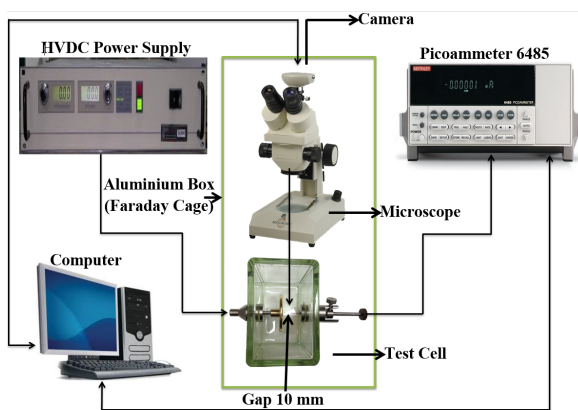
Fig. 1. Complete block diagram of experimental setup under influence of DC electric field with needle plane electrodes [2].
