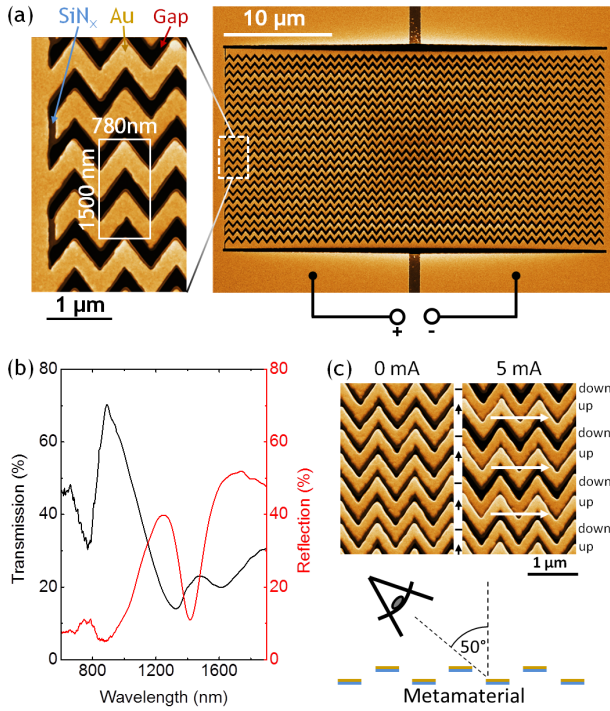
FIG. 2: Reconfigurable photonic metamaterial.
