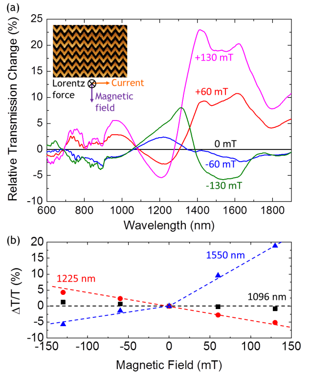
FIG. 4: Magnetic tuning. (a) Spectral dependence of the relative transmission change resulting from application of various magnetic fields to the metamaterial device while a constant 4 mA current is applied. The applied magnetic field and the electric field of the incident wave are directed perpendicular to the plasmonic metamaterial bridges in the metamaterial plane. (b) Relative transmission change as function of applied magnetic field for characteristic wavelengths. Quasi-linear and saturation regimes are indicated by dashed lines.
