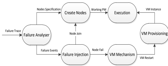
Figure 2. DesktopCloudSim Model
