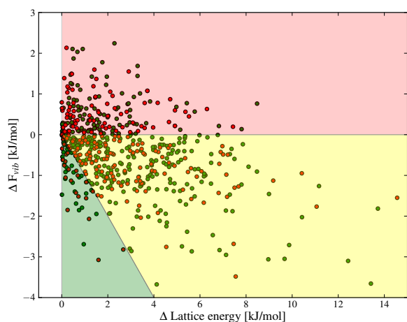
Fig. 4 Differences in lattice energy, E_{latt} , and total vibrational contributions to the free energy, F_{vib} , between polymorphs. The order of polymorphs is defined so that \Delta E_{latt} is positive in all cases. \Delta F_{vib} is calculated at T = 300 K. The shading indicates areas where \Delta E_{latt} and \Delta F_{vib} are the same sign (red), \Delta E_{latt} and \Delta F_{vib} are of opposite sign (yellow and green) and where \Delta F_{vib} causes a re-ordering of polymorph stability at 300 K (green). Green and red data points denote structures with and without hydrogen bonds, respectively.
