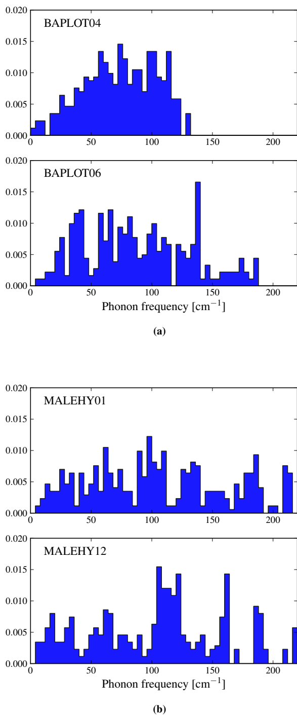
Fig. 7 The phonon density of states for a) theophylline polymorphs I and II and b) the two monoclinic polymorphs of maleic hydrazide. The target k-point sampling is 0.12 \text{ \AA}^{-1} in all cases.
