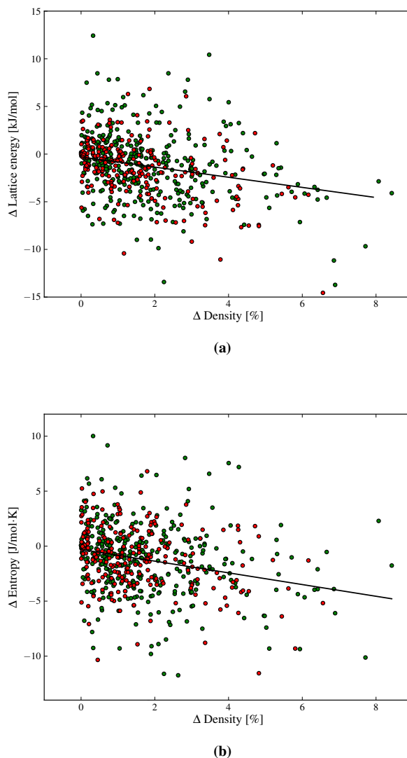
Fig. 8 Differences in a) lattice energy and b) entropy vs density differences between polymorphs. Polymorphs in each pair are ordered such that the density difference is positive. Green and red data points denote structures with and without hydrogen bonding. The correlation in both cases is statistically significant to p < 10^{-9} .
