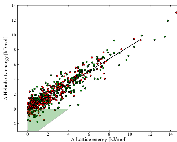
Fig. 9 The correlation between \Delta E_{latt} and \Delta A between polymorphs. Each polymorph pair is ordered such that the lattice energy difference is positive. The green area highlights those structures where re-ranking occurs between lattice energy and free energy at 300 K. Green and red data points denote structures with and without hydrogen bonds, respectively.
