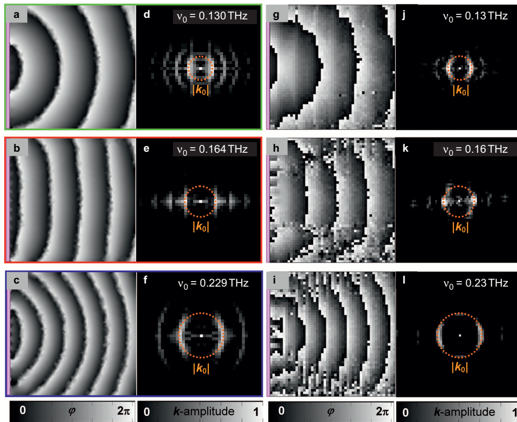
Figure 3. Wavefront transformation by ASR-based wavevector selective surface. (a–c) – Modeled spatial variations of the instantaneous phase, which visualize the wavefronts transmitted by the WSS at 0.130, 0.164 and 0.229 THz when it is illuminated by spherical waves. The waves originate from a vertically polarized point source/pinhole (not shown), on the left of the shaded purple bars, which represent the cross-section of the WSS. (d–f) – Spatial-frequency spectra of the wavefronts shown in panels (a–c) respectively. (g–i) – Experimentally measured spatial variation of the instantaneous phase, which visualizes the wavefront of the initially spherical waves transmitted by WSS at 0.13, 0.16, and 0.23 THz. (j–l) – Spatial-frequency spectra of the wavefront patterns shown in panels (g–i), correspondingly.
