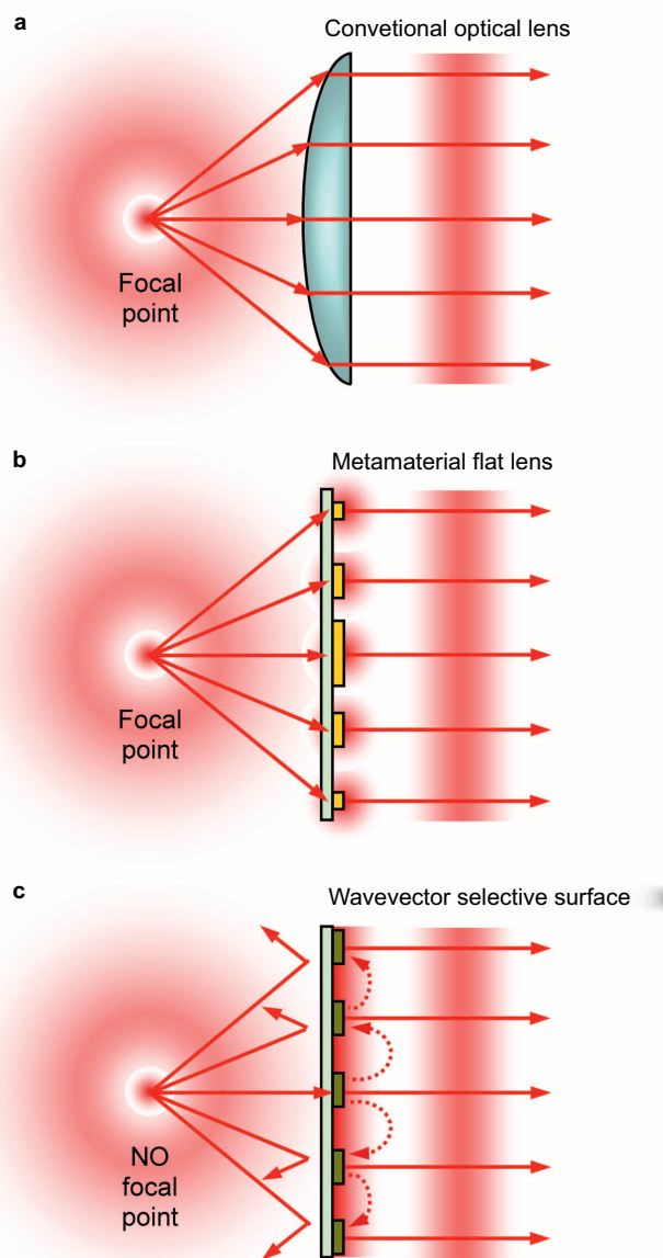
Figure 1. Three ways of producing planar wavefronts with a point light source.
