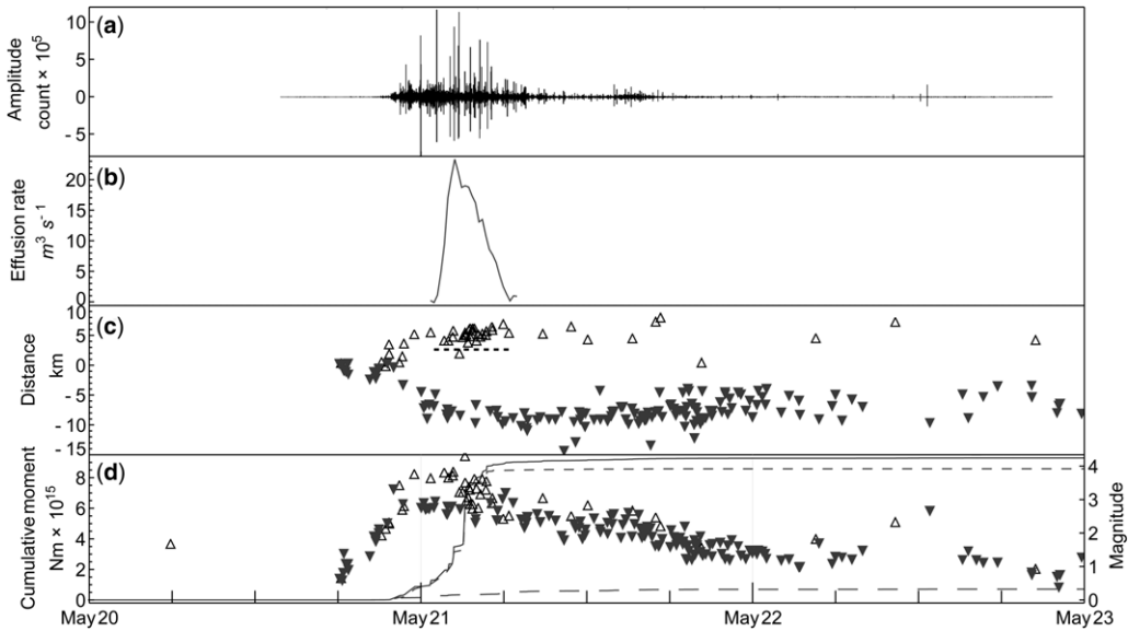
Fig. 5. The timing of seismic events and lava effusion. (a) Vertical component seismic trace for station IGR (see Fig. 1a). (b) Effusion rate calculated from extracted SEVIRI band 3 ( 1.6 \mu\text{m} ) radiance. (c) Migration of seismicity along dyke by distance from centre. Open triangles are northern segment earthquakes, filled triangles southern segment earthquakes and dashed line shows location and duration of the eruption. All earthquakes within 3 km of the dyke are plotted. (d) Earthquake magnitudes and cumulative moment for all events within 3 km of the dyke model. Open triangles are earthquakes in the northern dyke segment, filled triangles in the southern dyke segment, short dashed line shows cumulative seismic moment for northern dyke, long dashed line is for southern dyke and the continuous line gives the total.
