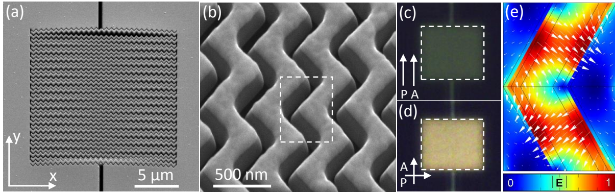
Figure 2. Suspended zig-zag metasurface. (a) SEM micrograph of the fabricated sample. (b) SEM micrograph of a small fragment of the metasurface taken at 52^\circ to the structure's normal. Dashed box indicates elementary unit cell of zig-zag pattern. (c) & (d) Images of liquid crystal-loaded metasurface in a twisted cell configuration made under a polarization optical microscope in transmission. Arrows indicate mutual orientations of the microscope's polarizer P and analyzer A . Dashed boxes indicate the area of the cell occupied by the metasurface. (e) Distribution of the amplitude of induced electric field calculated in the plane of bare metasurface at the resonant wavelength of 1.2 \mu\text{m} . White arrows show instantaneous direction of induced electric field.
