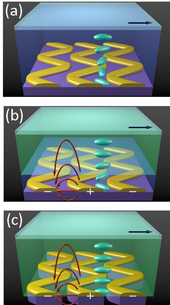
Figure 1. Schematic impression of a hybrid liquid-crystal cell with nano-structured metasurface electrically controlled via in-plane potentials. (a) OFF state of the cell featuring initially twisted ordering in the bulk of the liquid crystal layer. (b) ON state of the cell: liquid crystal ordering has been switched to planar (green) except for a very thin layer at the bottom (blue) with residual twist due to strong surface anchoring. (c) ON state of the cell with suspended metasurface: switching from twisted to planar state is complete both in the bulk and in the plane of the metasurface. Black arrow indicates the direction of rubbing that sets liquid crystal alignment at the top cover.
