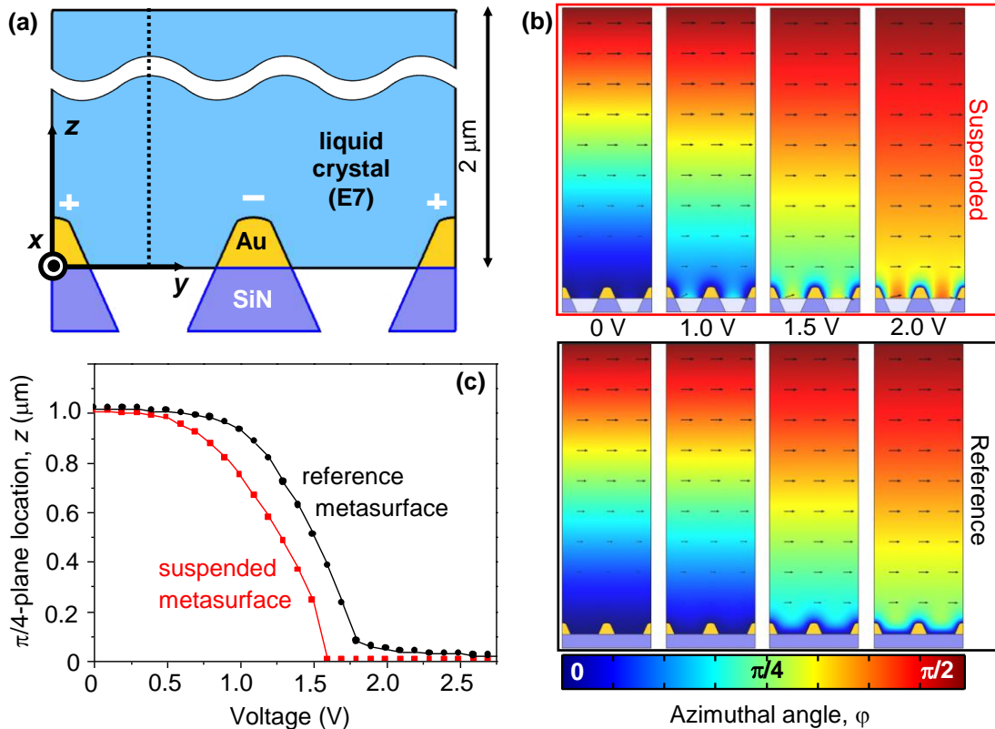
Figure 4. Electrically induced elastic distortions of liquid crystal in hybrid twisted cells. (a) Schematic of the simulation domain representing a two-period wide cross-section of the hybrid cell with suspended metasurface. (b) Spatially dependent orientation of LC-director above suspended and reference metasurfaces calculated for 0, 1.0, 1.5 and 2.0 V of the potential difference applied between their nano-wires. Colour maps show spatial variations of the director's azimuthal angle \phi , where \phi = 0 and \phi = \pi/2 correspond to the director being orthogonal and parallel to the plane respectively. Arrows represent local projections of the director onto the plane of the plot. (c) Location of the effective interface between planar and twisted liquid crystal (the \phi = \pi/4 plane) as a function of applied voltage. Propagation of the interface was evaluated along the vertical cross-section indicated in panel (a) by the dashed line.
