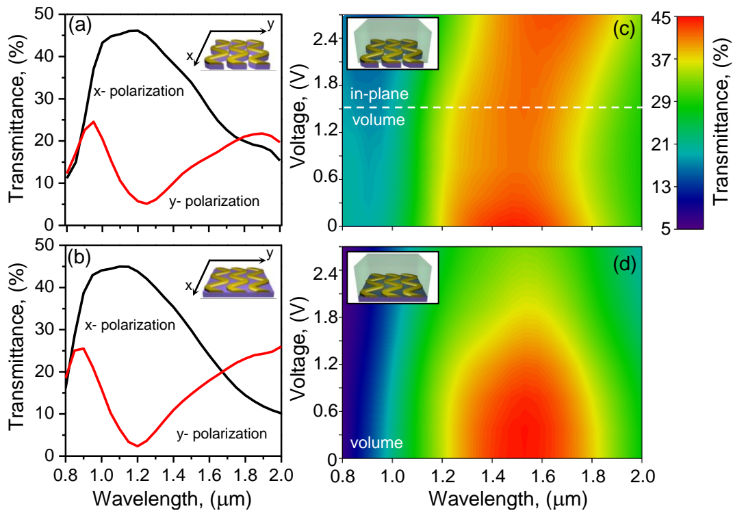
Figure 3. Electrically tunable near-IR response of zig-zag metasurfaces. (a) & (b) Transmission spectra of correspondingly suspended and reference bare metasurfaces measured for x - and y -polarization. (c) & (d) Transmittance of hybrid liquid-crystal cells with correspondingly suspended and reference metasurfaces measured for x -polarization as a function of wavelength and potential difference applied between zig-zag nano-wires. Dashed line indicates the transition between two regimes of electrical tuning corresponding to volume and in-plane switching of the hybrid cell.
