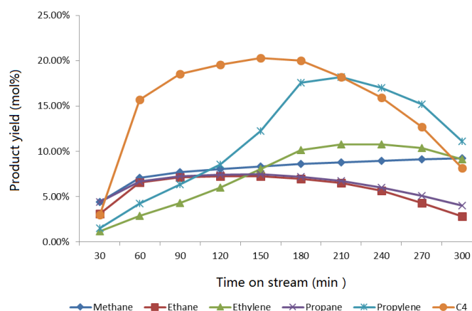
Fig. 10c The evolution of various gas products with time on-stream over 7.5 wt% MoO 3 /H-ZSM-5 at a temperature of 400 °C, atmosphere pressure
