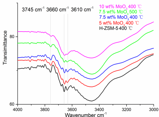
Fig. 4 Fourier Transform - IR spectra of hydroxyl group regions on the parent H-ZSM-5 and \text{MoO}_3 -loaded samples prepared at 400^\circ\text{C}/500^\circ\text{C}
