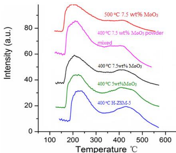
Fig. 6 \text{NH}_3 – Temperature Programmed Desorption profiles of \text{MoO}_3/\text{H-ZSM-5} samples prepared via different conditions (impregnation/powder mixing, 400\text{--}500^\circ\text{C} ) together with the original H-ZSM-5 sample ( 400^\circ\text{C} )
