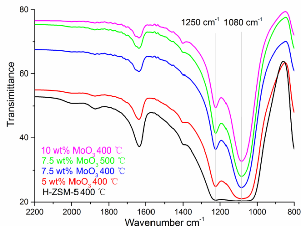
Fig. 5 Fourier Transform - IR spectra of H-ZSM-5 samples with different \text{MoO}_3 loading levels prepared at 400^\circ\text{C}/500^\circ\text{C}
