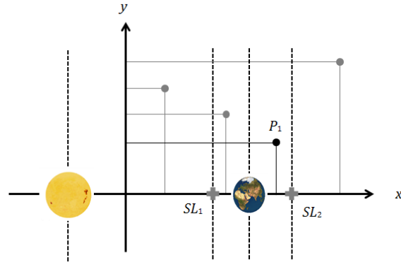
Figure 6: Reference system for studying the closure in SL_j .
