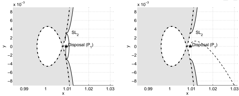
(a) EOL disposal with SRP. The \beta required is 0.02499. (b) After the closure the spacecraft is at the right-hand side of SL_2 .
