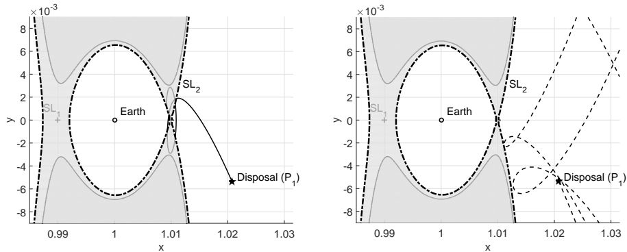
(c) Deployment of a Sun-pointing area in P_1 to close the zero-velocity poyment in P_1 , black dashed is inter-curved in SL_2 . (d) Trajectory evolution after the deployment in P_1 , black dashed is integrated for 63.5 years.
