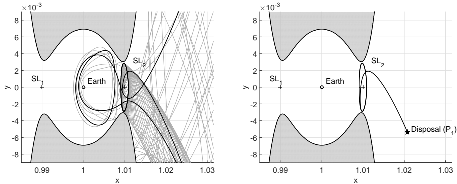
(a) Unstable manifold: the highlighted trajectory encounters the Earth after 29.5 years. (b) Selected trajectory where the deployment is done after 68.04 days from the leaving LPO.
