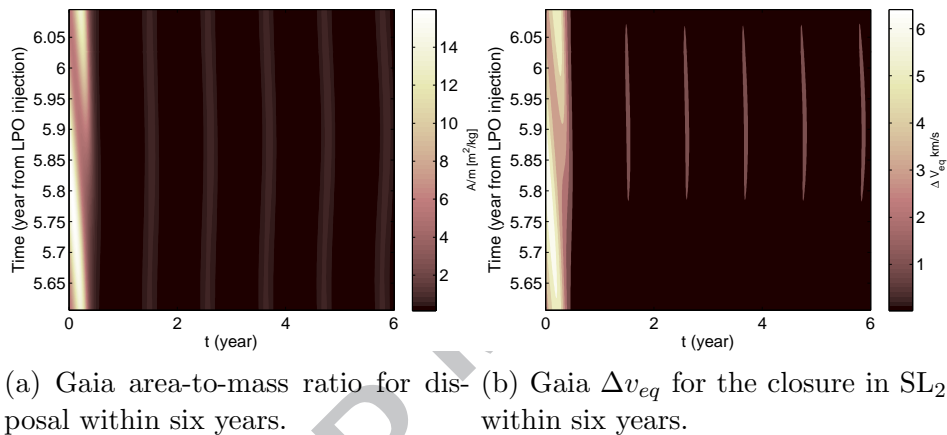
Figure 8: Gaia area-to-mass ratio and equivalent \Delta v_{eq} , figure from Colombo et al. (2014).
