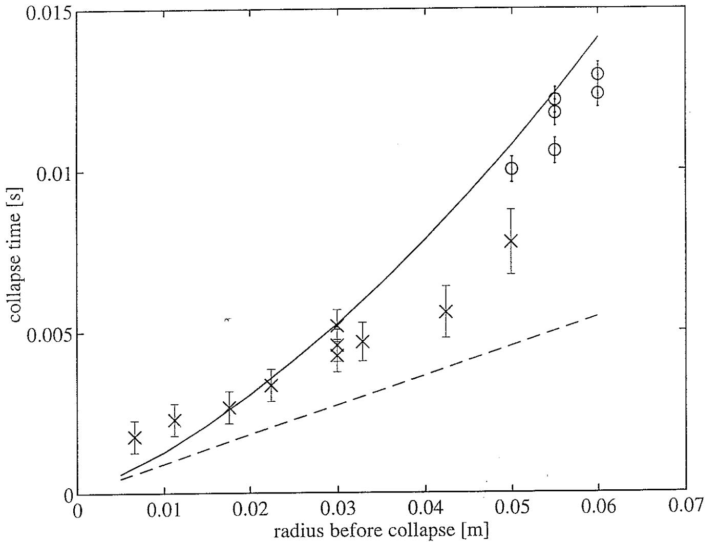
Figure 7. Plots of the collapse time of: (i) a gas-filled conical bubble (solid, found through integration of equation (3)), and (ii) an empty spherical Rayleigh cavity (dashed, equation (2)). The estimates of collapse times from data are shown, calculated from records of the pressure in the liquid (x), and from extrapolation from the high-speed images of the rebounds (o). In all the collapses from which these measurements were taken R_f = 0.95 \pm 0.05 mm and the device contained 1050 ml of degassed water ( h_i = 37.1 cm).
