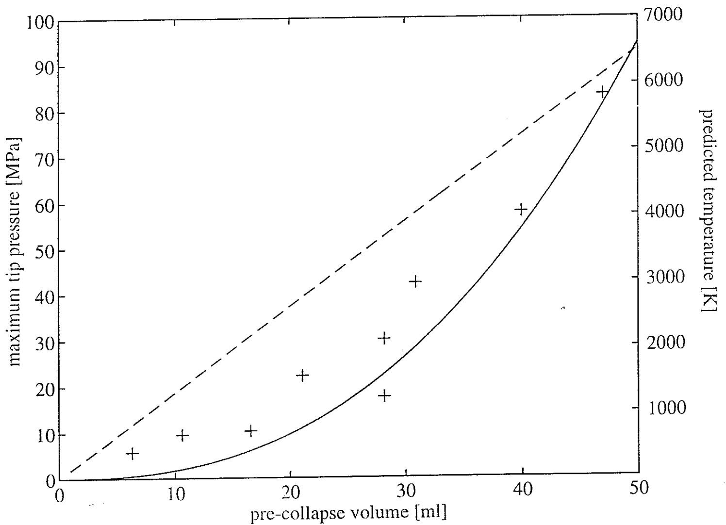
Figure 8. Measurements of pressure taken 5.1 mm below the apex of the cone, and spatially averaged across the cross-section. Predictions of theory for pressure are shown (equation (8), solid line). Also shown are predicted temperatures which would occur under these conditions (equation (9), broken line). The device contained 1050 ml of degassed water, the pre-growth bubble volume was 0.9 ml.
