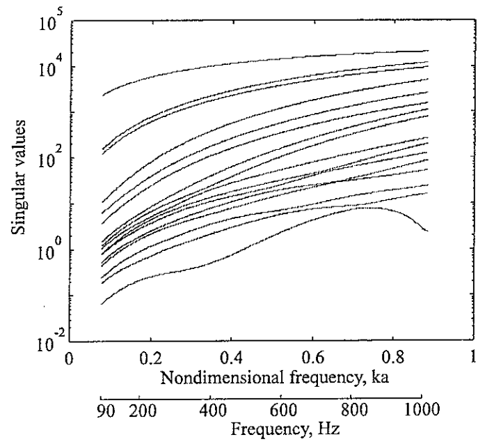
Figure 28. Singular values of the matrix \mathbf{H} for the model of Figure 16. a=L_x/8 , L_x=0.38\text{m} .
