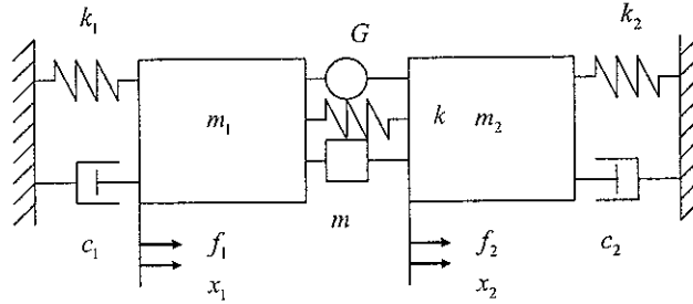
Figure C.1. Two general, conservatively coupled oscillators
