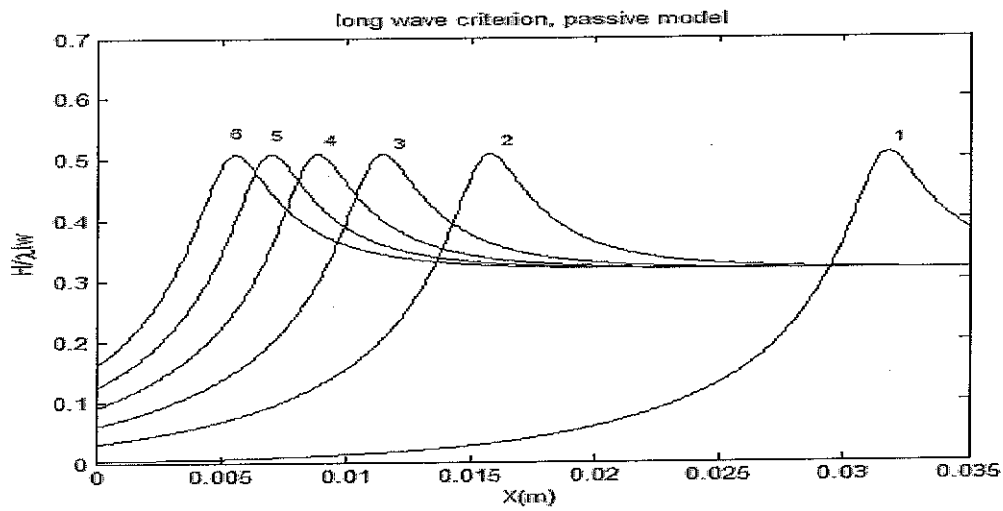
Figure 25: Long wave criterion using de Boer passive model (1, 2, 3, 4, 5, 6 correspond to 200 Hz, 2200 Hz, 4200 Hz, 6200 Hz, 8200 Hz, 10200 Hz respectively)
