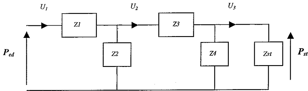
Figure 38: Block diagram for the middle ear
