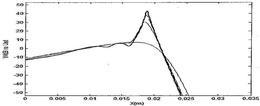
Figure 21: Velocity of the cochlear partition (amplitude and phase) for the locally active long wave model of Neely and Kim, the effect of varying the cochlear amplifier gain \gamma at 1000 Hz, ( \gamma=0 ; 1; 1.1 and 1.15), at this frequency “instabilities” appear for \gamma=1.15 .
