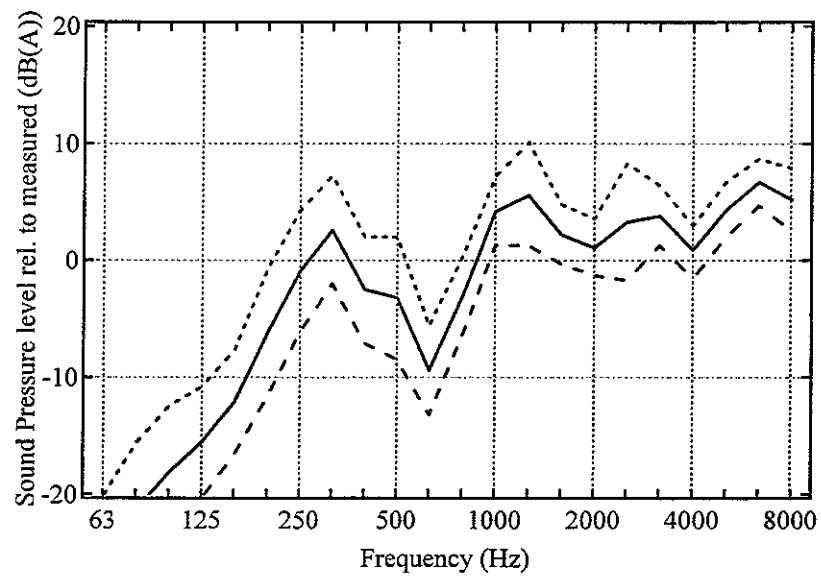
Figure D2.6 Average difference between predicted and measured noise spectra for all cases ( tinif, bi-bloc sleeper, —:mean, .....:mean+std deviation, - - - :mean-std deviation )
