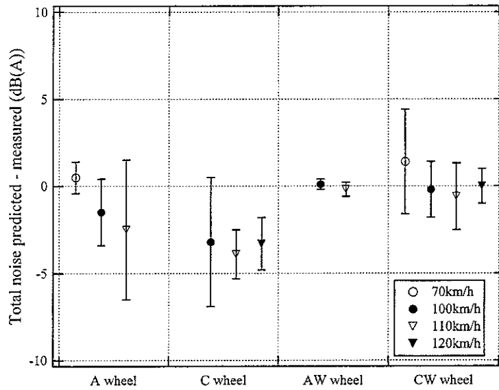
Figure 5.3 Total predicted noise minus measured noise in dB(A) (rodol, bi-bloc sleeper, results are shown for 70, 100, 110 and 110 km/h)
