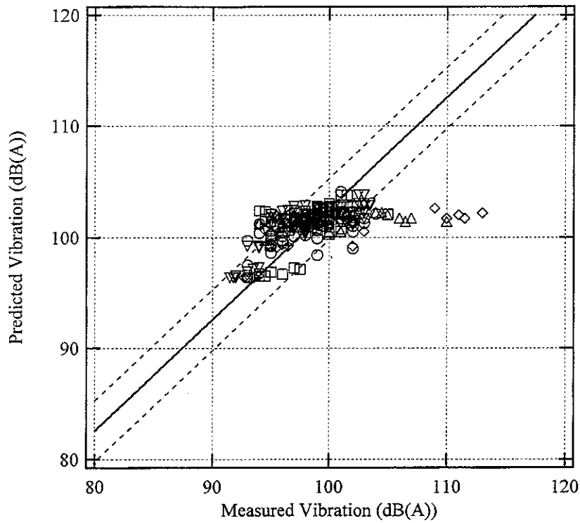
Figure E2.4 Predicted rail vibration velocity plotted against measured rail vibration velocity for all cases (vertical direction, tinj , mono-bloc sleeper)
