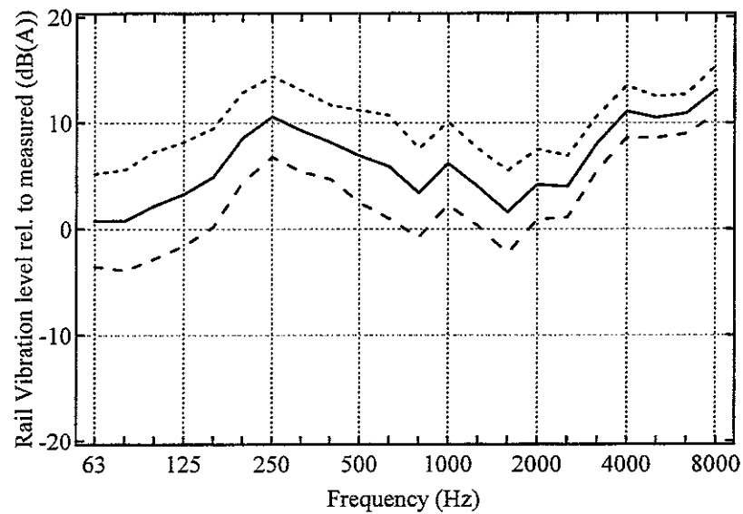
Figure E2.5 Average difference between predicted and measured rail vibration velocity spectra for all cases ( tinj , mono-bloc sleeper, — :mean, - - - :mean+std deviation, - . - :mean-std deviation, vertical direction)
