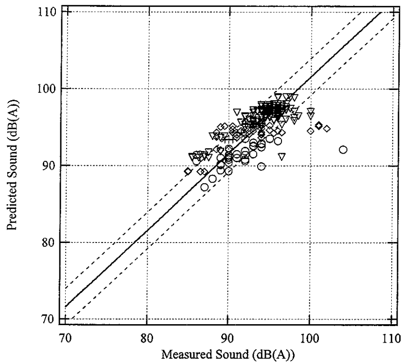
Figure D2.5 Predicted noise plotted against measured noise for all cases ( tinif, bi-bloc sleeper )
