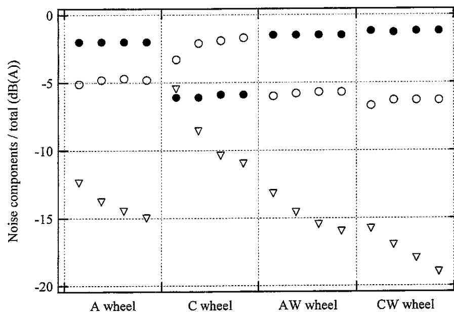
Figure D1.2 Predicted noise components from rail (○), wheel (●) and sleeper (▽) using rodel model (bi-bloc sleeper), minus predicted total noise in dB(A) Results are shown for each speed (70, 100, 110 and 120 km/h).
