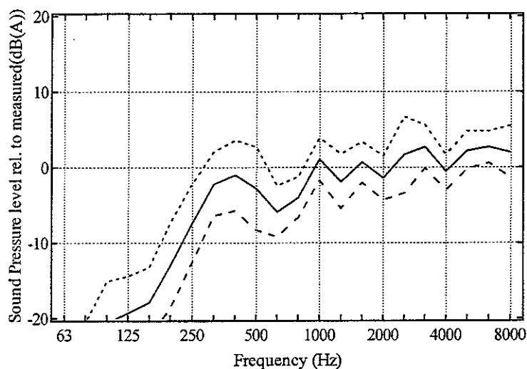
Figure 5.5 Average differences between predicted and measured noise spectra for all cases.
